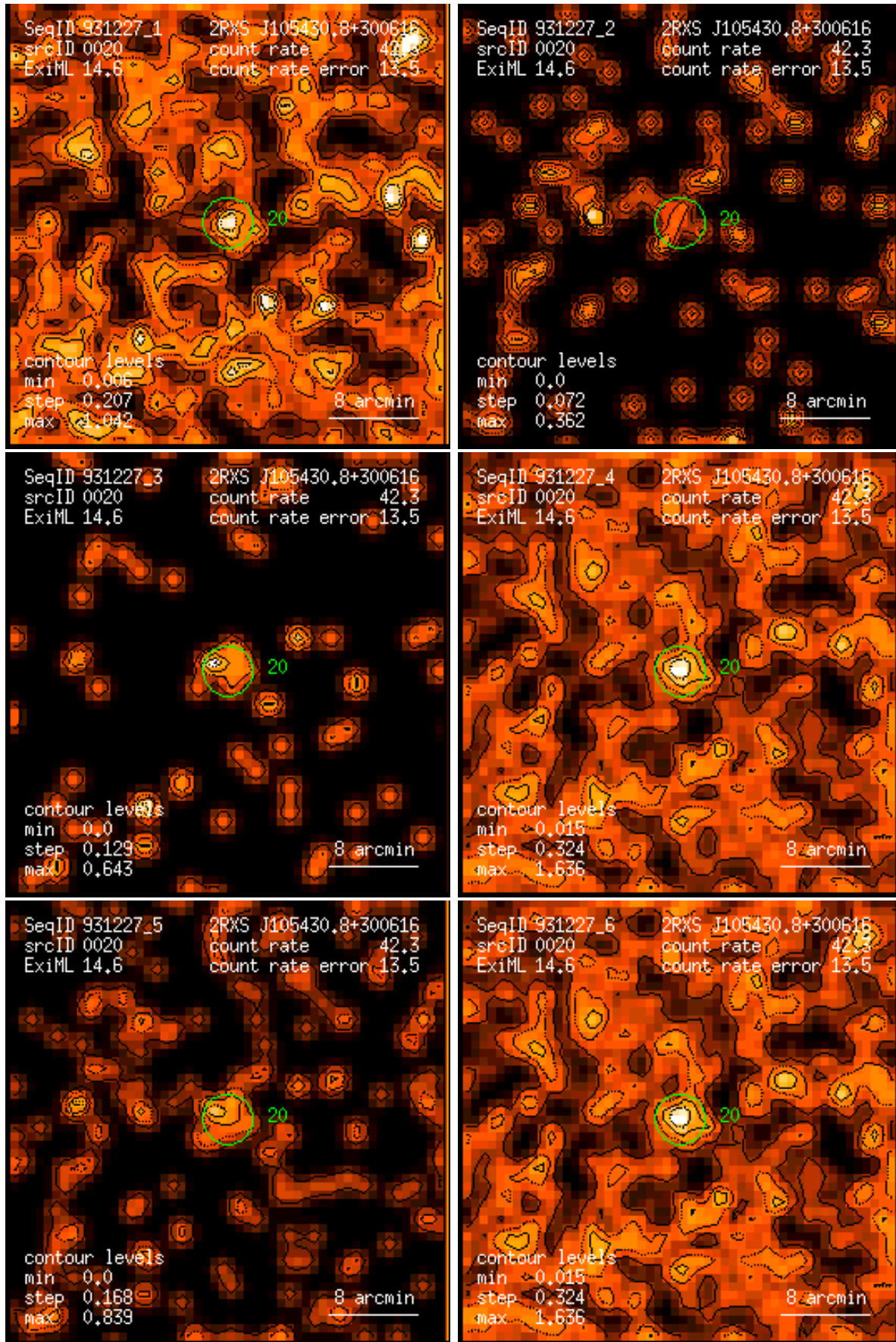
Figure 20: RASS 931227: detection 0020: band rate images, Gaussian filter: (1) PSPC channels 11 – 41, (2) 52 – 90, (3) 91 – 201, (4) 11 – 235, (5) 52 – 201, (6) 11 – 201. Broad band rates in counts/ks. Band rate contour levels in counts/ks/arcmin 2 .
