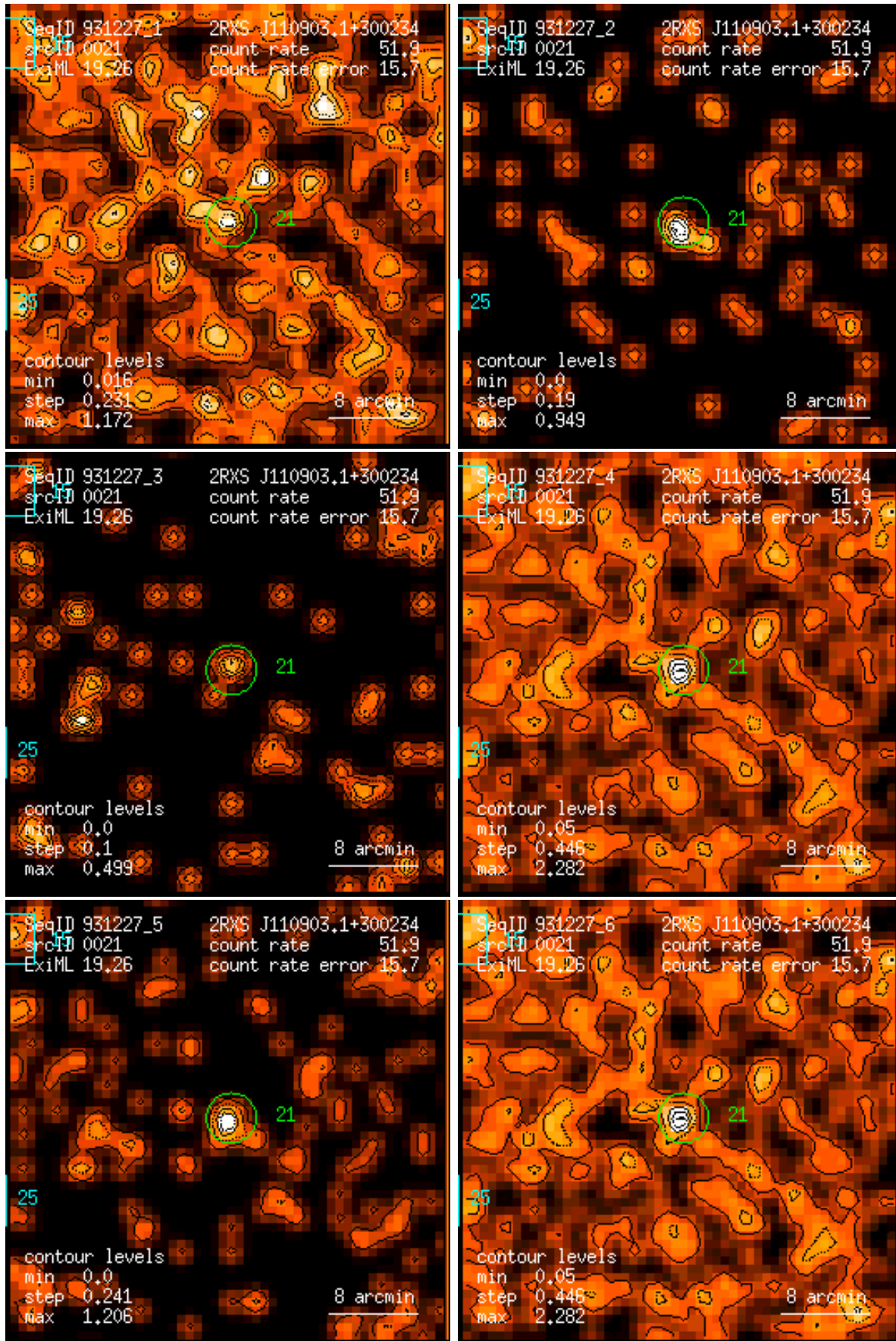
Figure 21: RASS 931227: detection 0021: band rate images, Gaussian filter: (1) PSPC channels 11 – 41, (2) 52 – 90, (3) 91 – 201, (4) 11 – 235, (5) 52 – 201, (6) 11 – 201. Broad band rates in counts/ks. Band rate contour levels in counts/ks/arcmin 2 .
