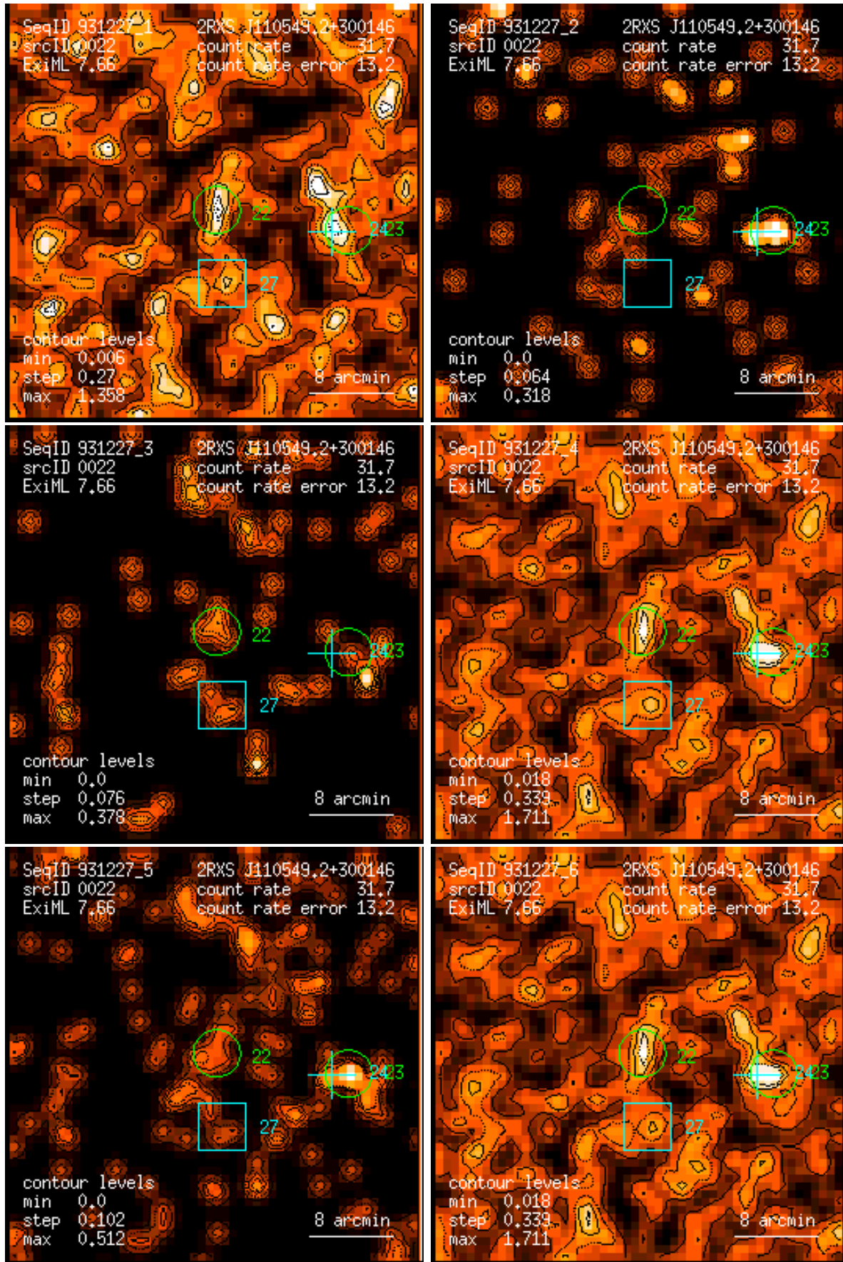
Figure 22: RASS 931227: detection 0022: band rate images, Gaussian filter: (1) PSPC channels 11 – 41, (2) 52 – 90, (3) 91 – 201, (4) 11 – 235, (5) 52 – 201, (6) 11 – 201. Broad band rates in counts/ks. Band rate contour levels in counts/ks/arcmin 2 .
