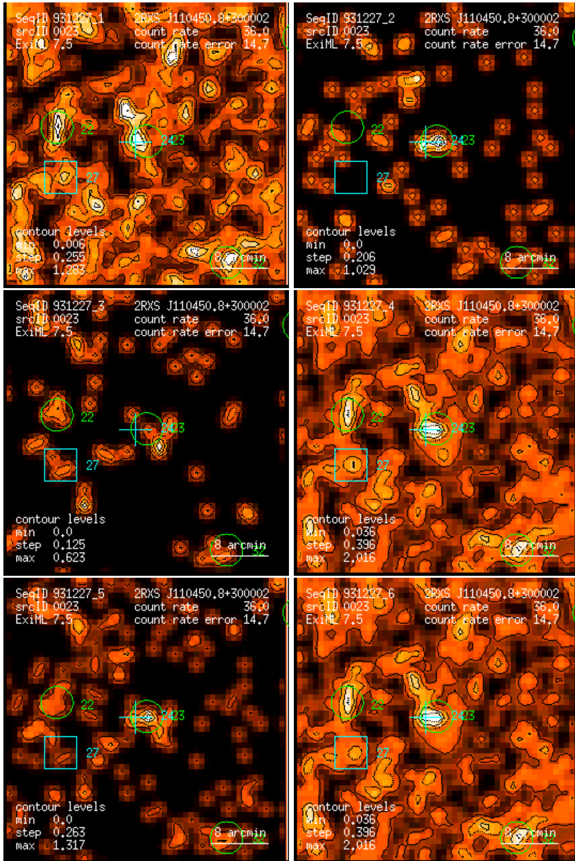
Figure 23: RASS 931227: detection 0023: band rate images, Gaussian filter: (1) PSPC channels 11 – 41, (2) 52 – 90, (3) 91 – 201, (4) 11 – 235, (5) 52 – 201, (6) 11 – 201. Broad band rates in counts/ks. Band rate contour levels in counts/ks/arcmin 2 .
