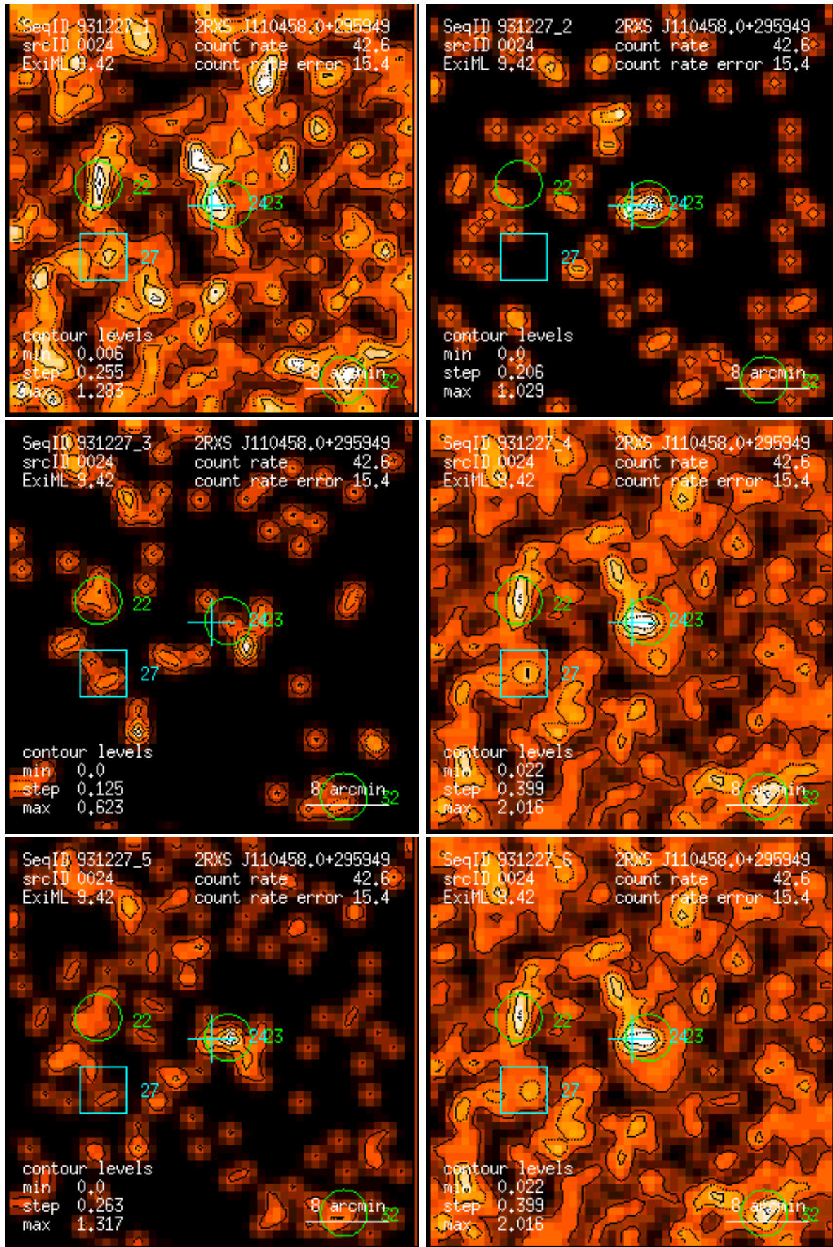
Figure 24: RASS 931227: detection 0024: band rate images, Gaussian filter: (1) PSPC channels 11 – 41, (2) 52 – 90, (3) 91 – 201, (4) 11 – 235, (5) 52 – 201, (6) 11 – 201. Broad band rates in counts/ks. Band rate contour levels in counts/ks/arcmin 2 .
