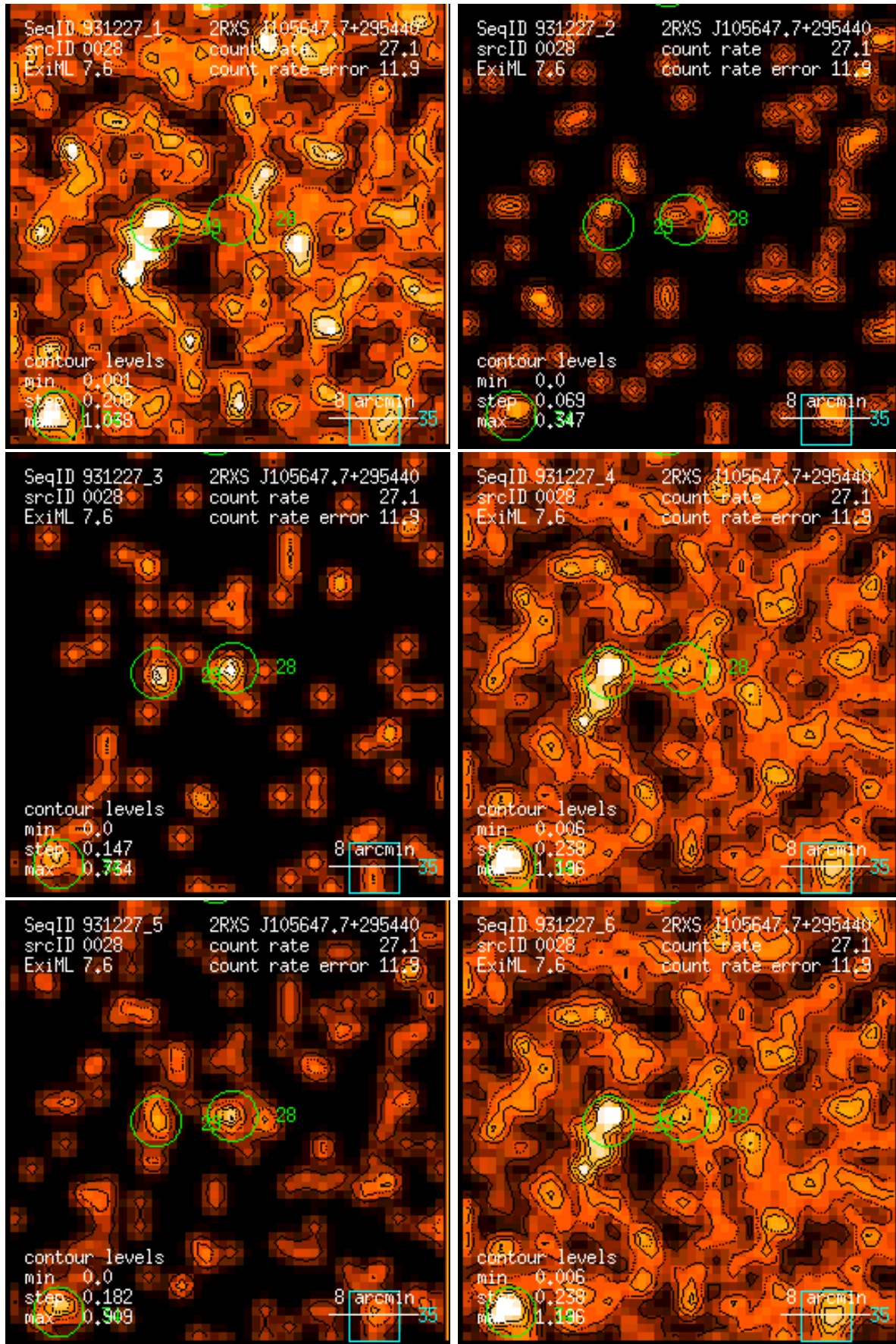
Figure 28: RASS 931227: detection 0028: band rate images, Gaussian filter: (1) PSPC channels 11 – 41, (2) 52 – 90, (3) 91 – 201, (4) 11 – 235, (5) 52 – 201, (6) 11 – 201. Broad band rates in counts/ks. Band rate contour levels in counts/ks/arcmin 2 .
