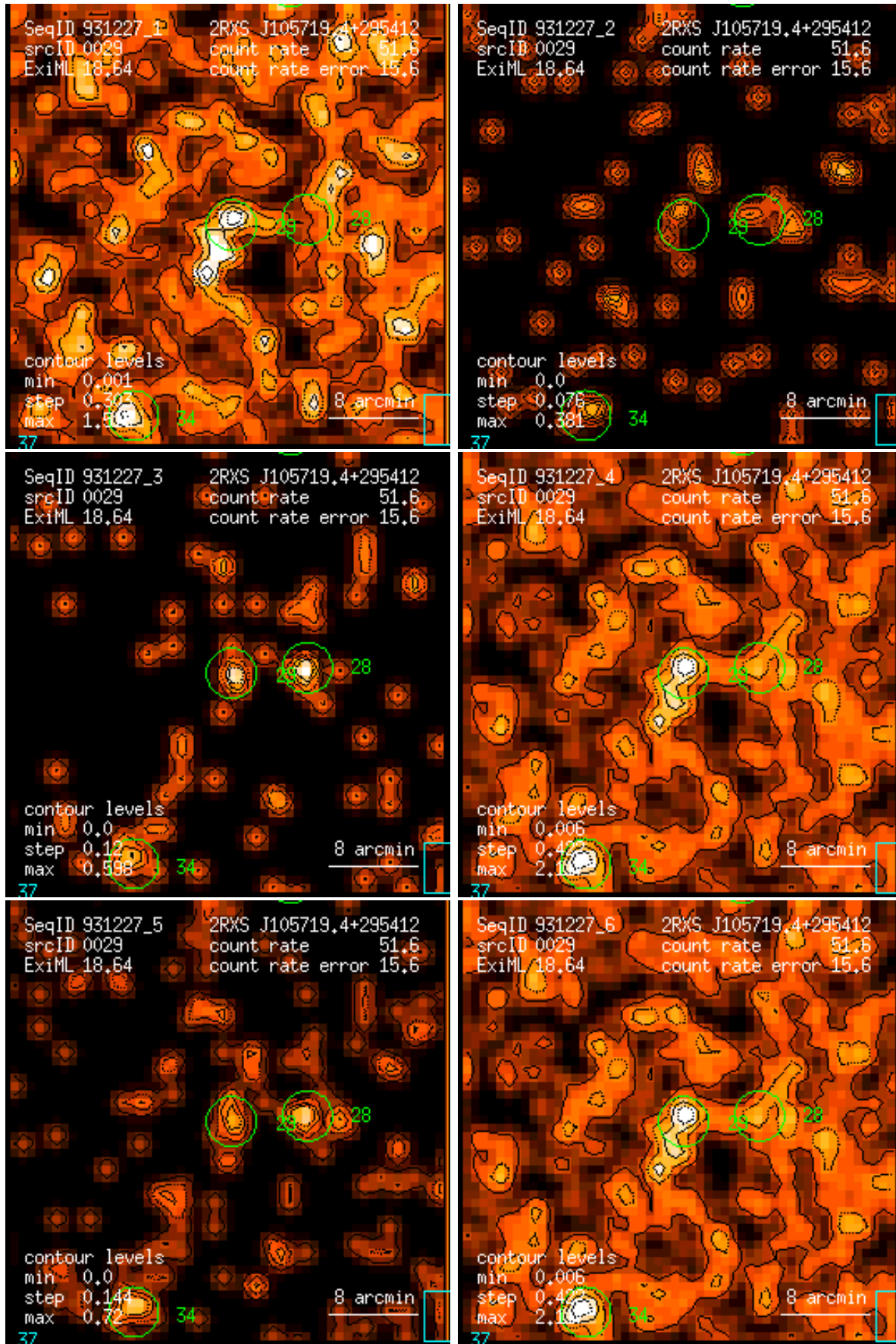
Figure 29: RASS 931227: detection 0029: band rate images, Gaussian filter: (1) PSPC channels 11 – 41, (2) 52 – 90, (3) 91 – 201, (4) 11 – 235, (5) 52 – 201, (6) 11 – 201. Broad band rates in counts/ks. Band rate contour levels in counts/ks/arcmin 2 .
