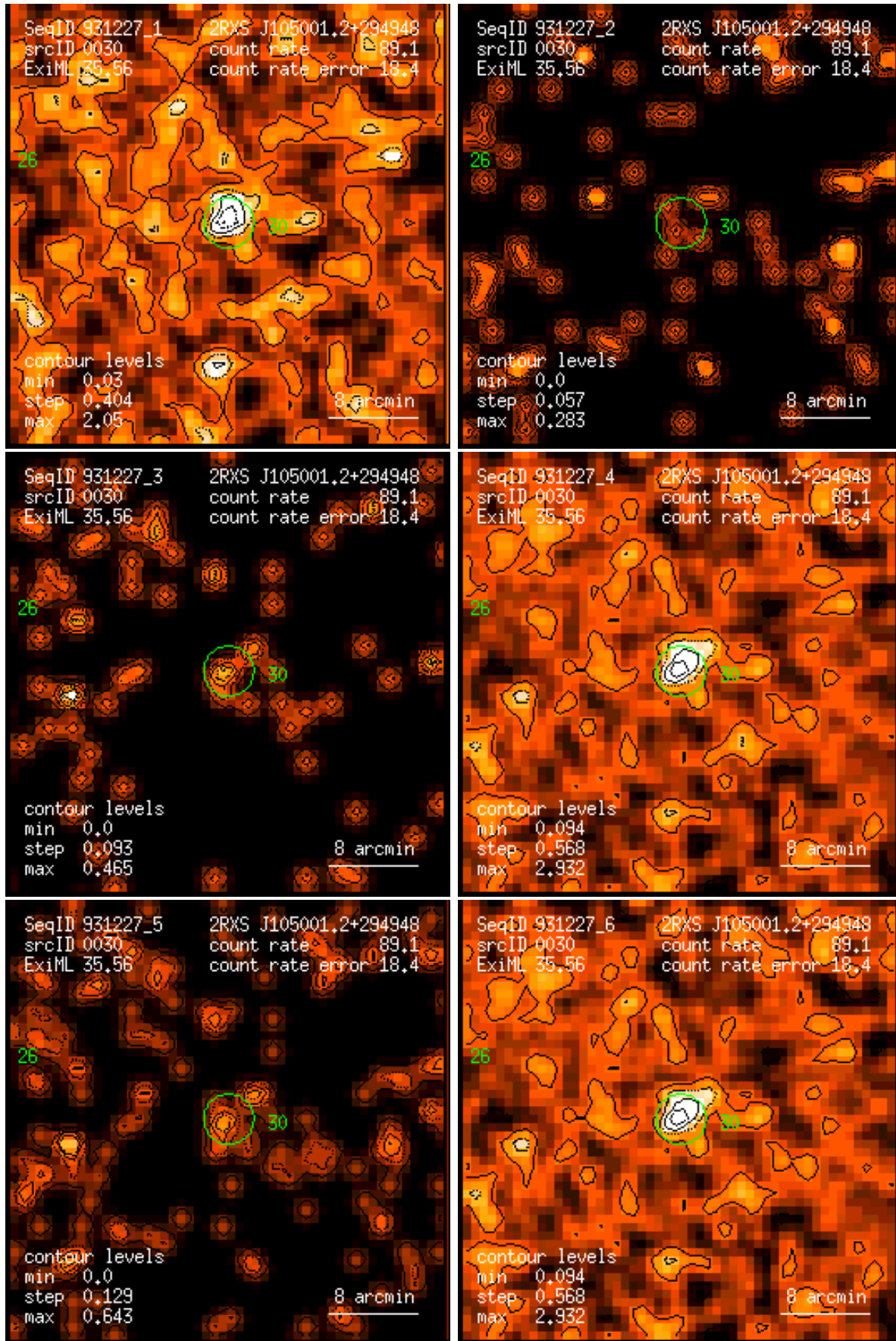
Figure 30: RASS 931227: detection 0030: band rate images, Gaussian filter: (1) PSPC channels 11 – 41, (2) 52 – 90, (3) 91 – 201, (4) 11 – 235, (5) 52 – 201, (6) 11 – 201. Broad band rates in counts/ks. Band rate contour levels in counts/ks/arcmin 2 .
