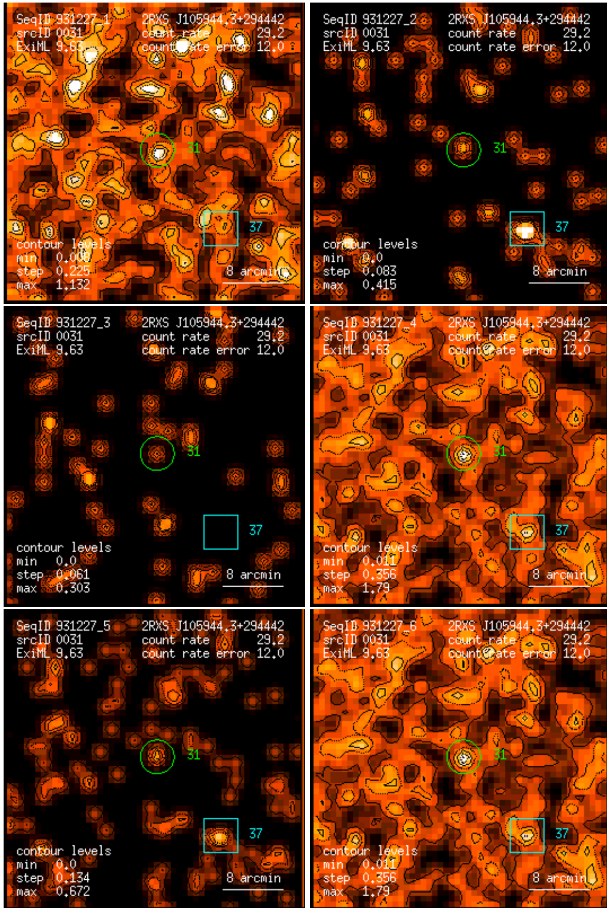
Figure 31: RASS 931227: detection 0031: band rate images, Gaussian filter: (1) PSPC channels 11 – 41, (2) 52 – 90, (3) 91 – 201, (4) 11 – 235, (5) 52 – 201, (6) 11 – 201. Broad band rates in counts/ks. Band rate contour levels in counts/ks/arcmin 2 .
