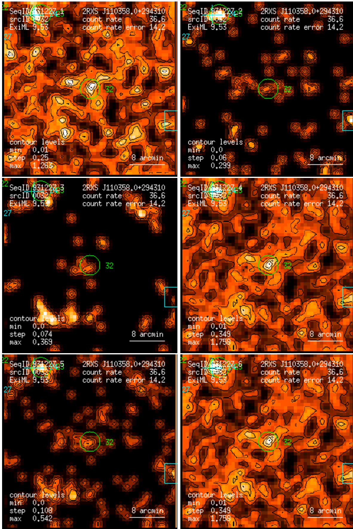
Figure 32: RASS 931227: detection 0032: band rate images, Gaussian filter: (1) PSPC channels 11 – 41, (2) 52 – 90, (3) 91 – 201, (4) 11 – 235, (5) 52 – 201, (6) 11 – 201. Broad band rates in counts/ks. Band rate contour levels in counts/ks/arcmin 2 .
