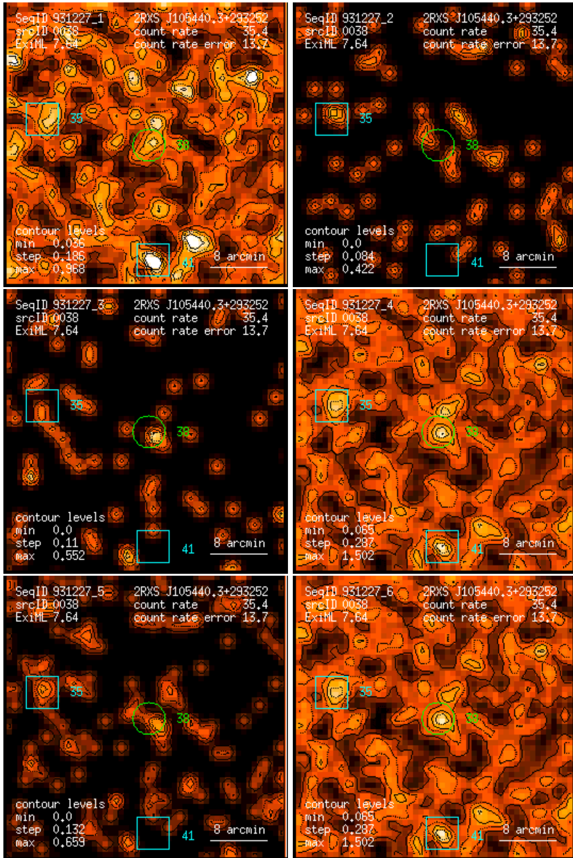
Figure 38: RASS 931227: detection 0038: band rate images, Gaussian filter: (1) PSPC channels 11 – 41, (2) 52 – 90, (3) 91 – 201, (4) 11 – 235, (5) 52 – 201, (6) 11 – 201. Broad band rates in counts/ks. Band rate contour levels in counts/ks/arcmin 2 .
