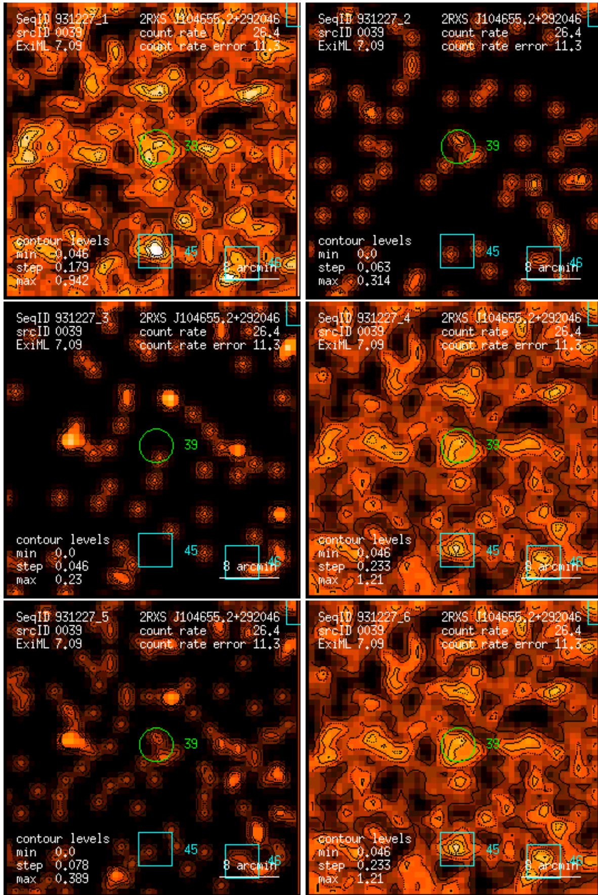
Figure 39: RASS 931227: detection 0039: band rate images, Gaussian filter: (1) PSPC channels 11 – 41, (2) 52 – 90, (3) 91 – 201, (4) 11 – 235, (5) 52 – 201, (6) 11 – 201. Broad band rates in counts/ks. Band rate contour levels in counts/ks/arcmin 2 .
