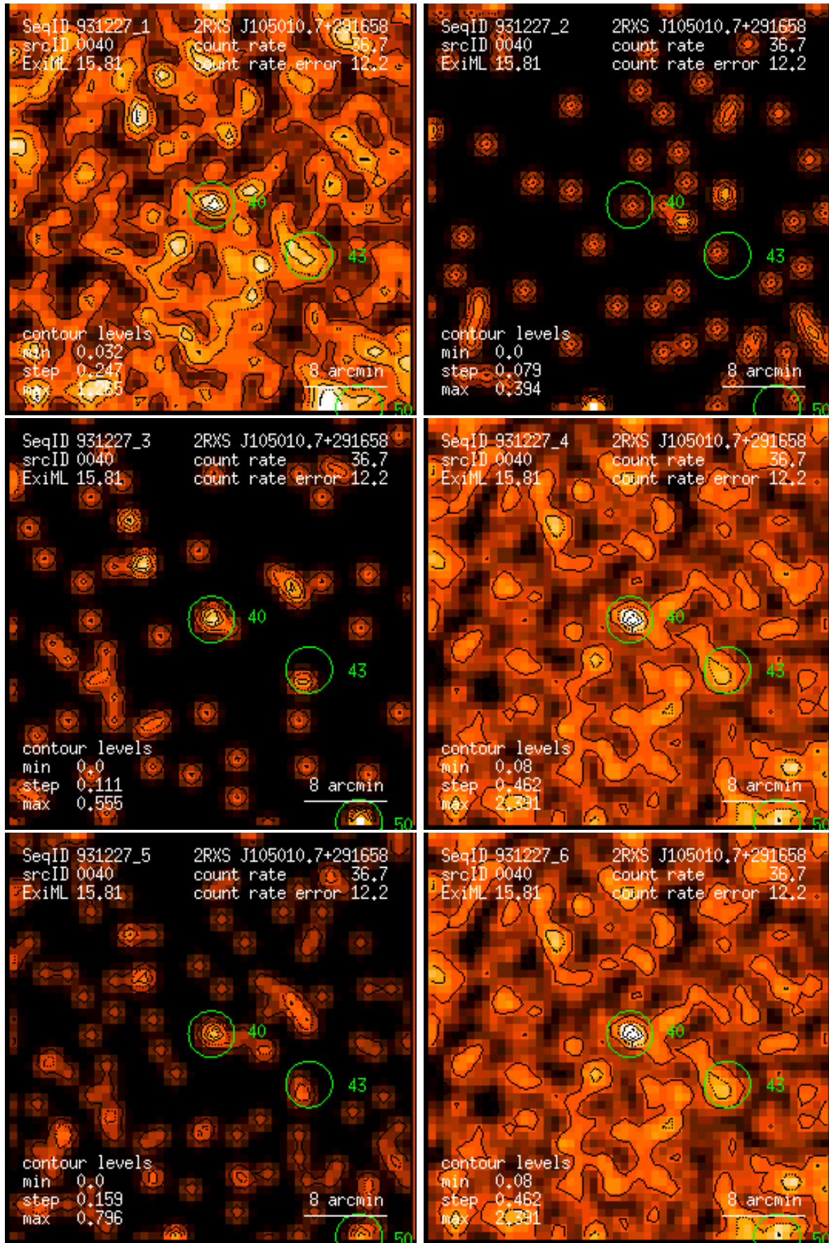
Figure 40: RASS 931227: detection 0040: band rate images, Gaussian filter: (1) PSPC channels 11 – 41, (2) 52 – 90, (3) 91 – 201, (4) 11 – 235, (5) 52 – 201, (6) 11 – 201. Broad band rates in counts/ks. Band rate contour levels in counts/ks/arcmin 2 .
