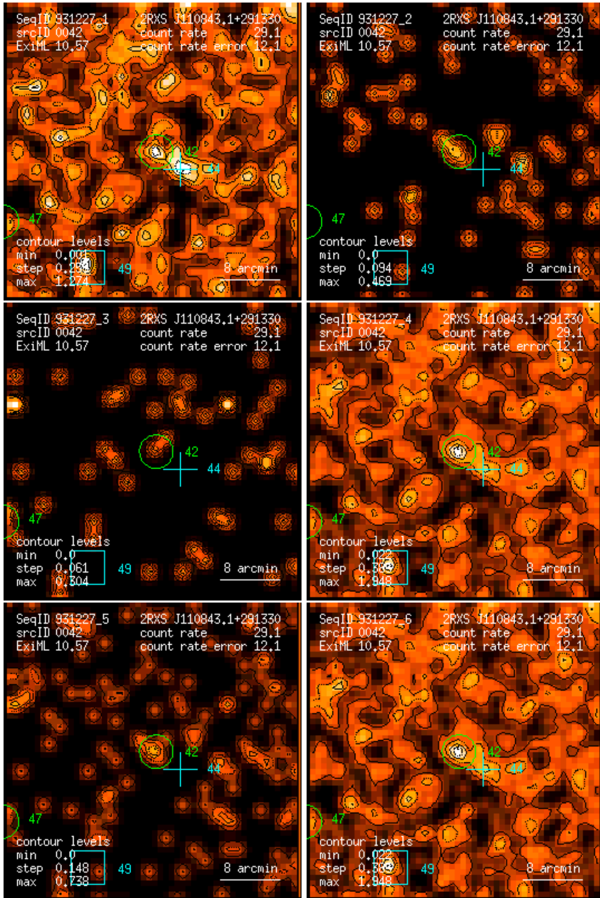
Figure 42: RASS 931227: detection 0042: band rate images, Gaussian filter: (1) PSPC channels 11 – 41, (2) 52 – 90, (3) 91 – 201, (4) 11 – 235, (5) 52 – 201, (6) 11 – 201. Broad band rates in counts/ks. Band rate contour levels in counts/ks/arcmin 2 .
