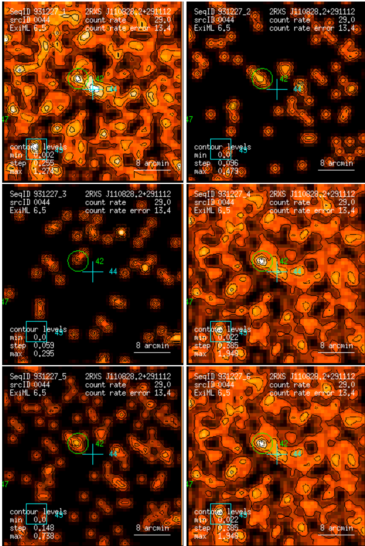
Figure 44: RASS 931227: detection 0044: band rate images, Gaussian filter: (1) PSPC channels 11 – 41, (2) 52 – 90, (3) 91 – 201, (4) 11 – 235, (5) 52 – 201, (6) 11 – 201. Broad band rates in counts/ks. Band rate contour levels in counts/ks/arcmin 2 .
