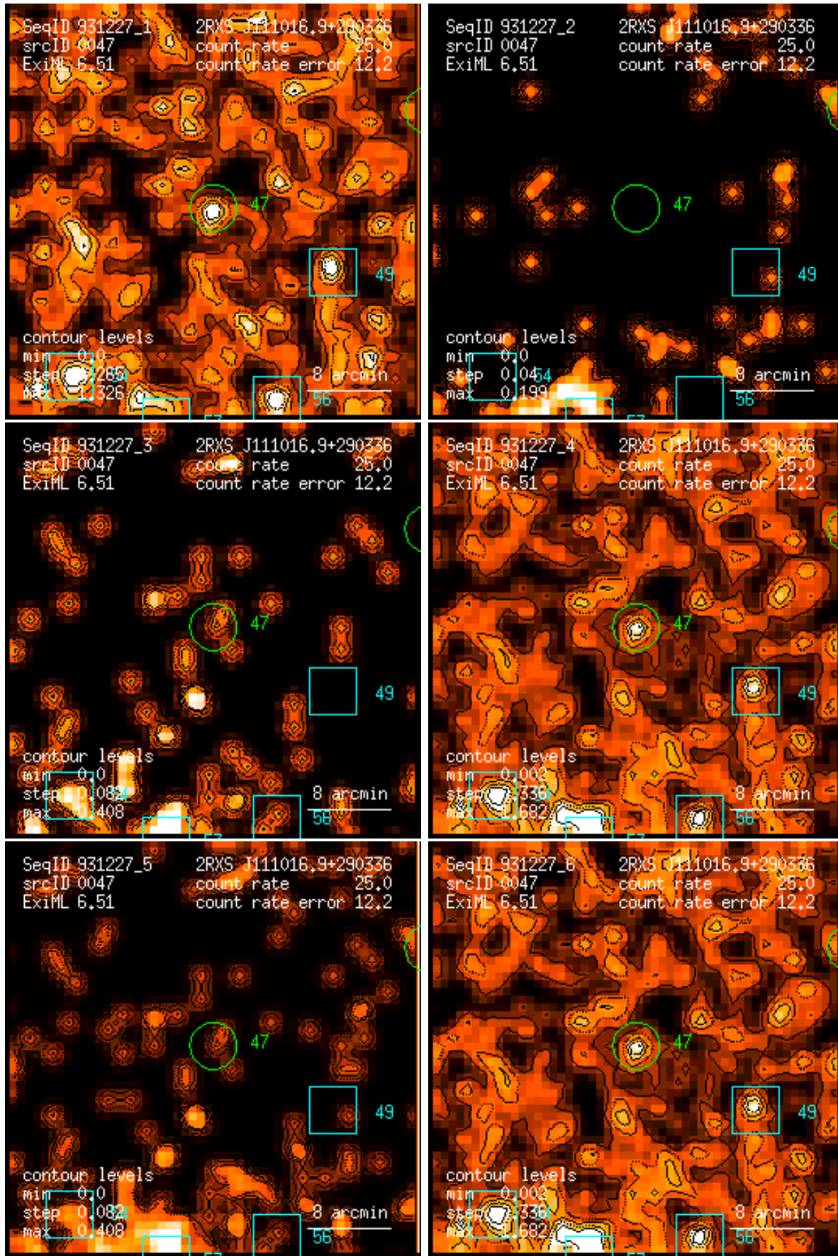
Figure 47: RASS 931227: detection 0047: band rate images, Gaussian filter: (1) PSPC channels 11 – 41, (2) 52 – 90, (3) 91 – 201, (4) 11 – 235, (5) 52 – 201, (6) 11 – 201. Broad band rates in counts/ks. Band rate contour levels in counts/ks/arcmin 2 .
