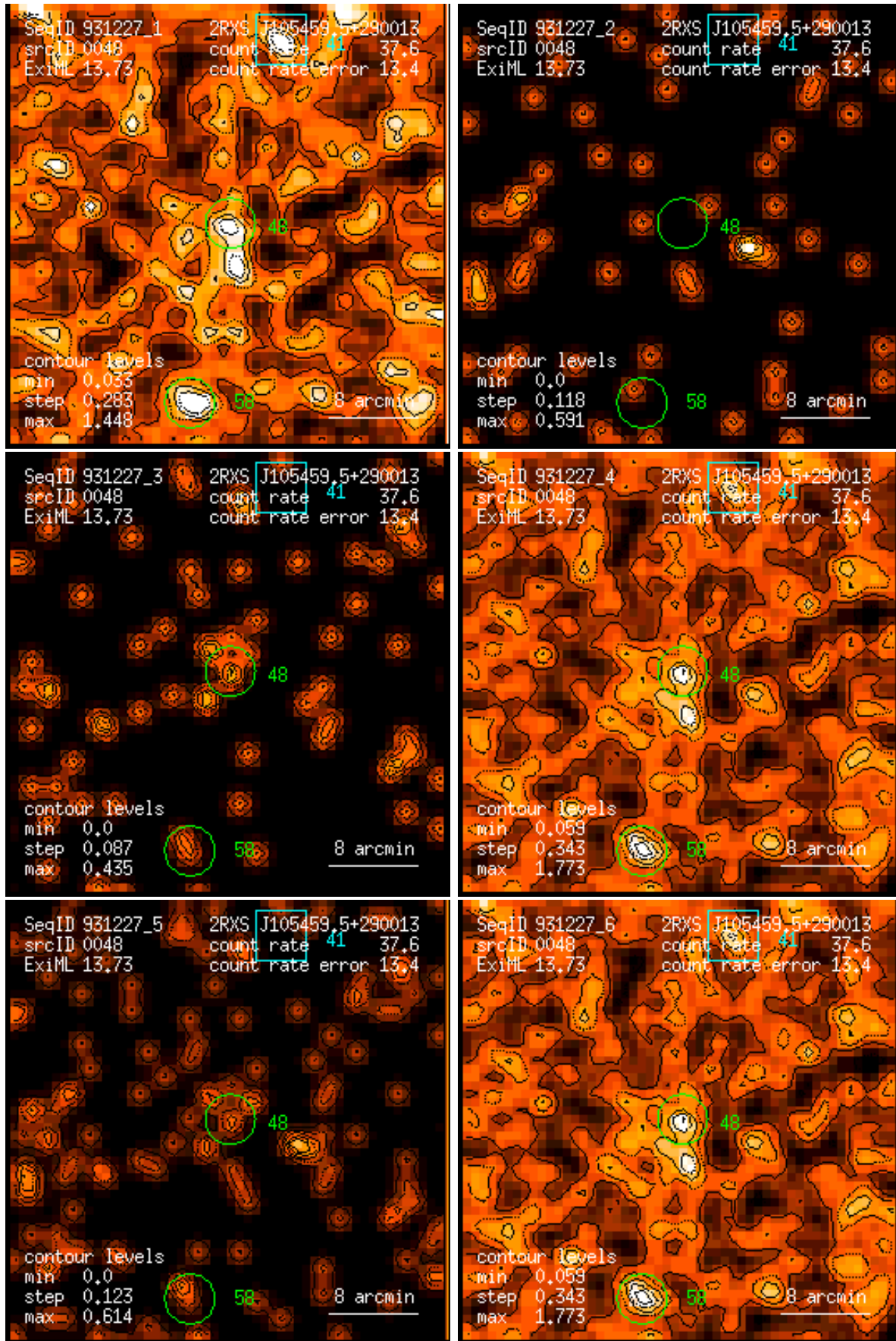
Figure 48: RASS 931227: detection 0048: band rate images, Gaussian filter: (1) PSPC channels 11 – 41, (2) 52 – 90, (3) 91 – 201, (4) 11 – 235, (5) 52 – 201, (6) 11 – 201. Broad band rates in counts/ks. Band rate contour levels in counts/ks/arcmin 2 .
