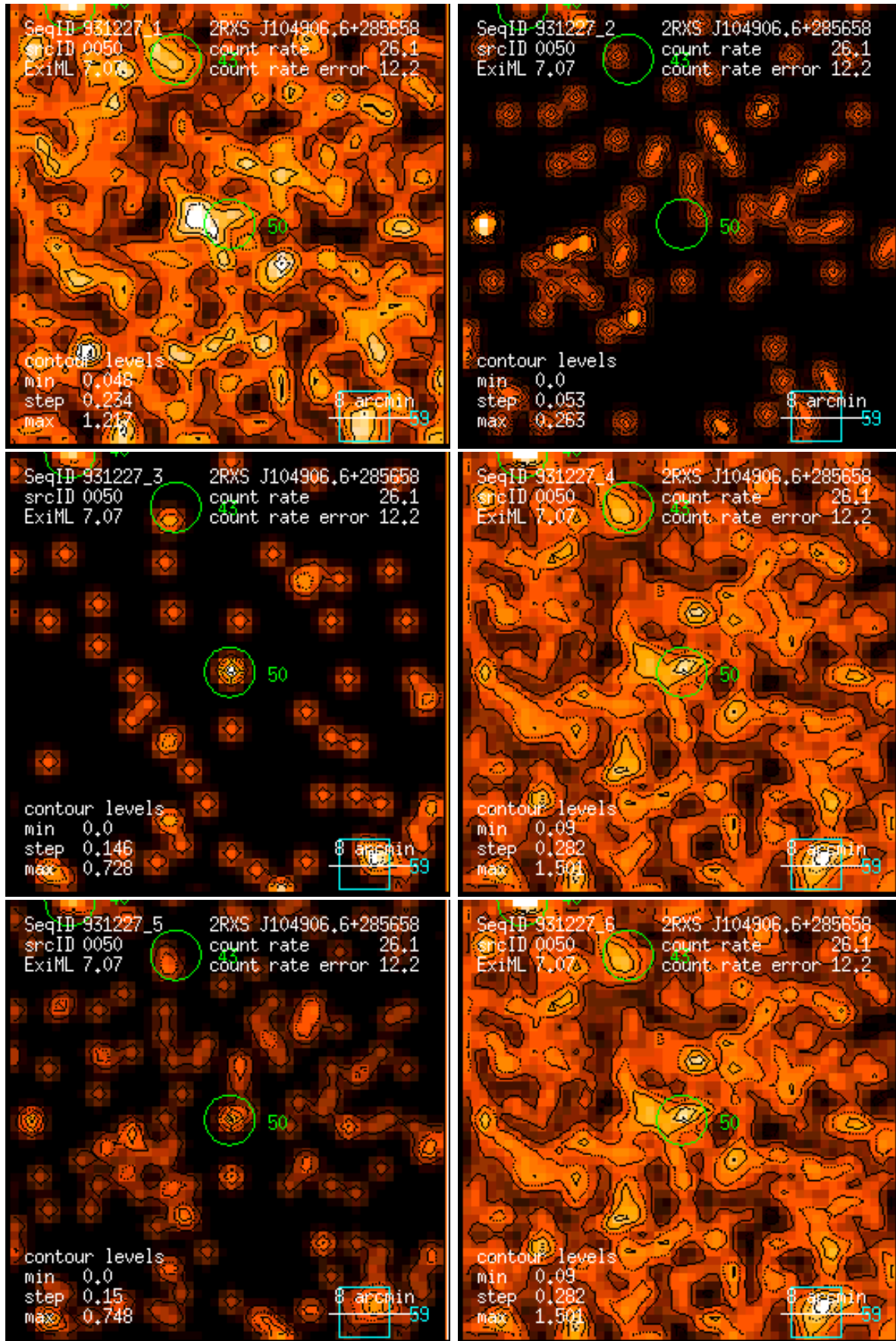
Figure 50: RASS 931227: detection 0050: band rate images, Gaussian filter: (1) PSPC channels 11 – 41, (2) 52 – 90, (3) 91 – 201, (4) 11 – 235, (5) 52 – 201, (6) 11 – 201. Broad band rates in counts/ks. Band rate contour levels in counts/ks/arcmin 2 .
