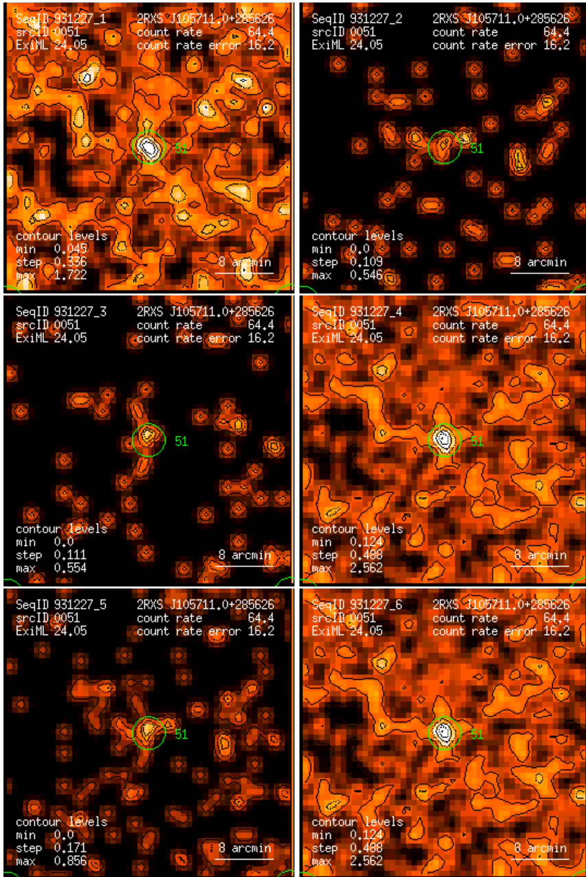
Figure 51: RASS 931227: detection 0051: band rate images, Gaussian filter: (1) PSPC channels 11 – 41, (2) 52 – 90, (3) 91 – 201, (4) 11 – 235, (5) 52 – 201, (6) 11 – 201. Broad band rates in counts/ks. Band rate contour levels in counts/ks/arcmin 2 .
