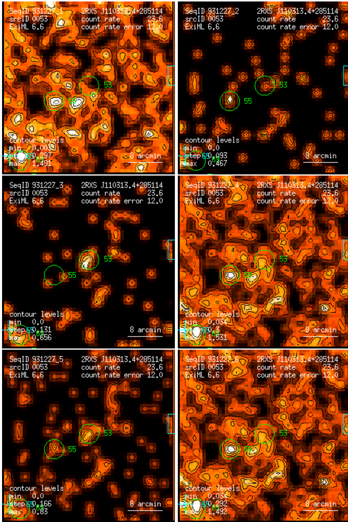
Figure 53: RASS 931227: detection 0053: band rate images, Gaussian filter: (1) PSPC channels 11 – 41, (2) 52 – 90, (3) 91 – 201, (4) 11 – 235, (5) 52 – 201, (6) 11 – 201. Broad band rates in counts/ks. Band rate contour levels in counts/ks/arcmin 2 .
