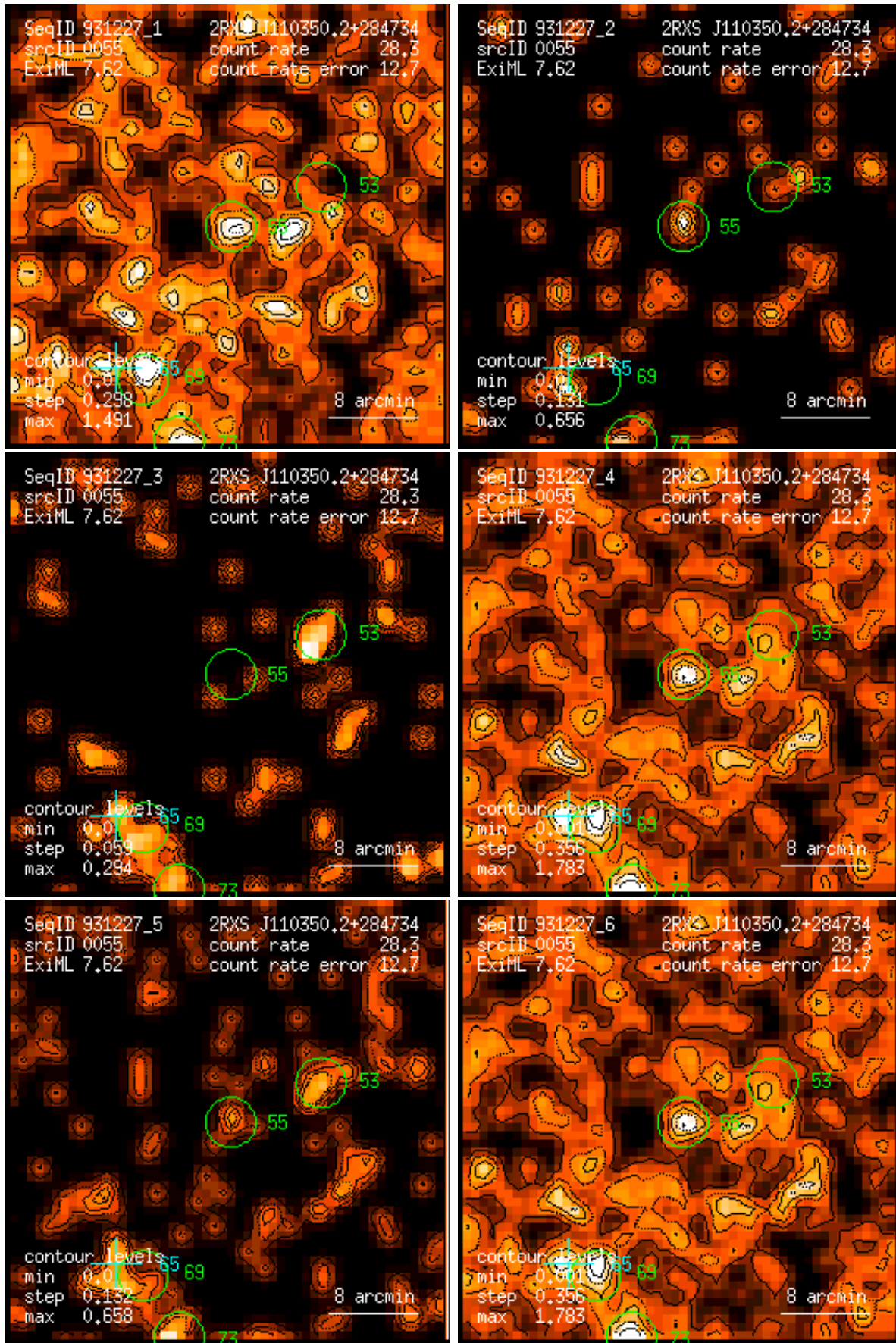
Figure 55: RASS 931227: detection 0055: band rate images, Gaussian filter: (1) PSPC channels 11 – 41, (2) 52 – 90, (3) 91 – 201, (4) 11 – 235, (5) 52 – 201, (6) 11 – 201. Broad band rates in counts/ks. Band rate contour levels in counts/ks/arcmin 2 .
