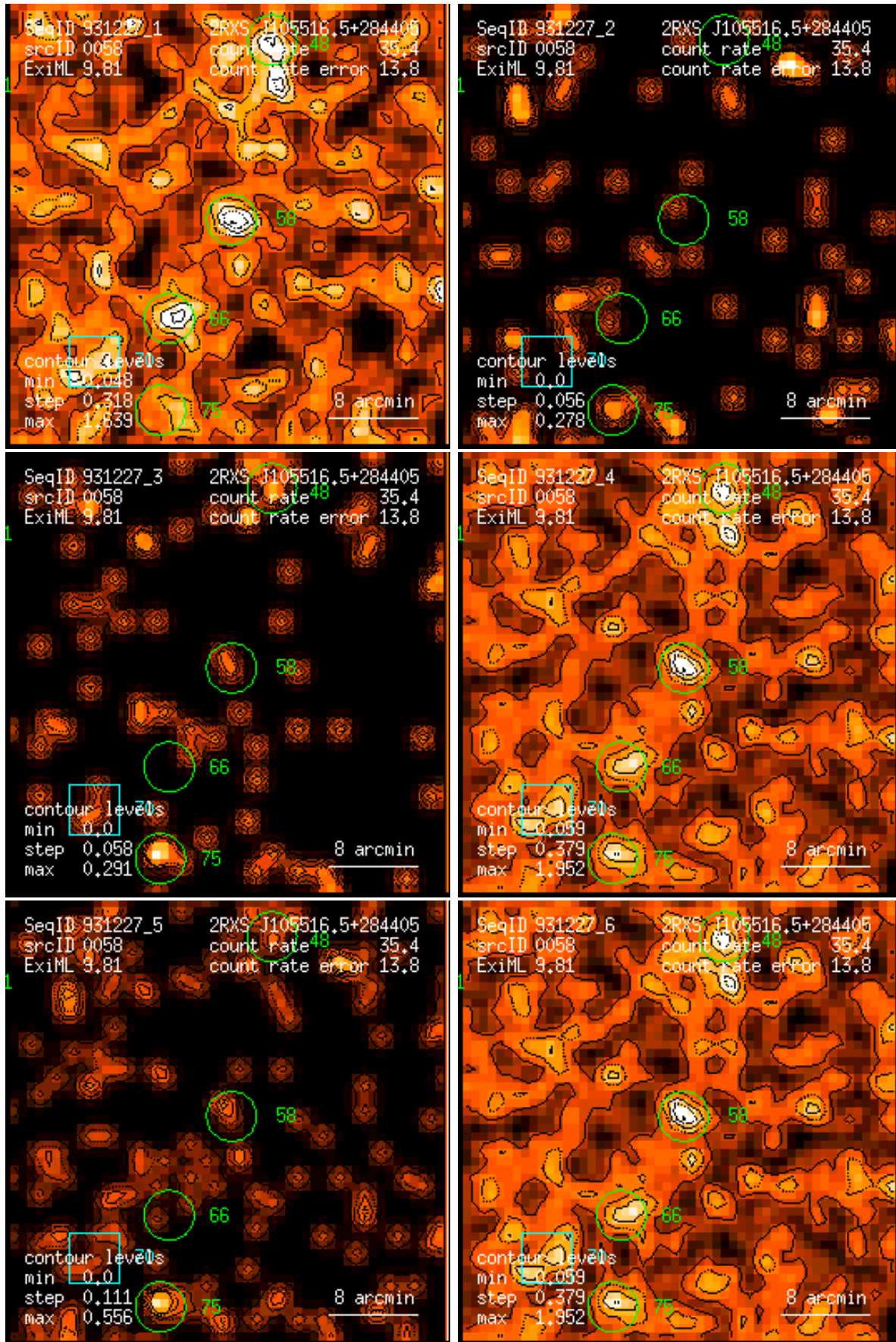
Figure 58: RASS 931227: detection 0058: band rate images, Gaussian filter: (1) PSPC channels 11 – 41, (2) 52 – 90, (3) 91 – 201, (4) 11 – 235, (5) 52 – 201, (6) 11 – 201. Broad band rates in counts/ks. Band rate contour levels in counts/ks/arcmin 2 .
