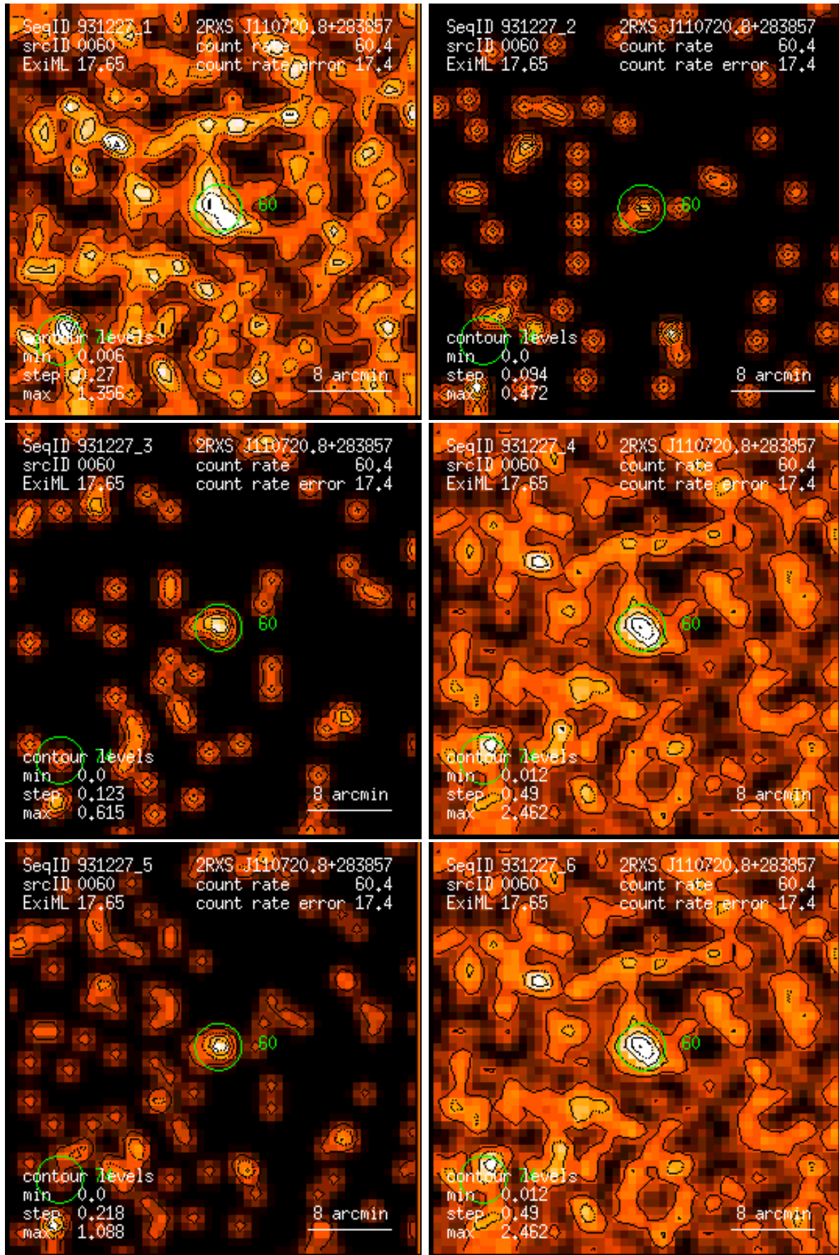
Figure 60: RASS 931227: detection 0060: band rate images, Gaussian filter: (1) PSPC channels 11 – 41, (2) 52 – 90, (3) 91 – 201, (4) 11 – 235, (5) 52 – 201, (6) 11 – 201. Broad band rates in counts/ks. Band rate contour levels in counts/ks/arcmin 2 .
