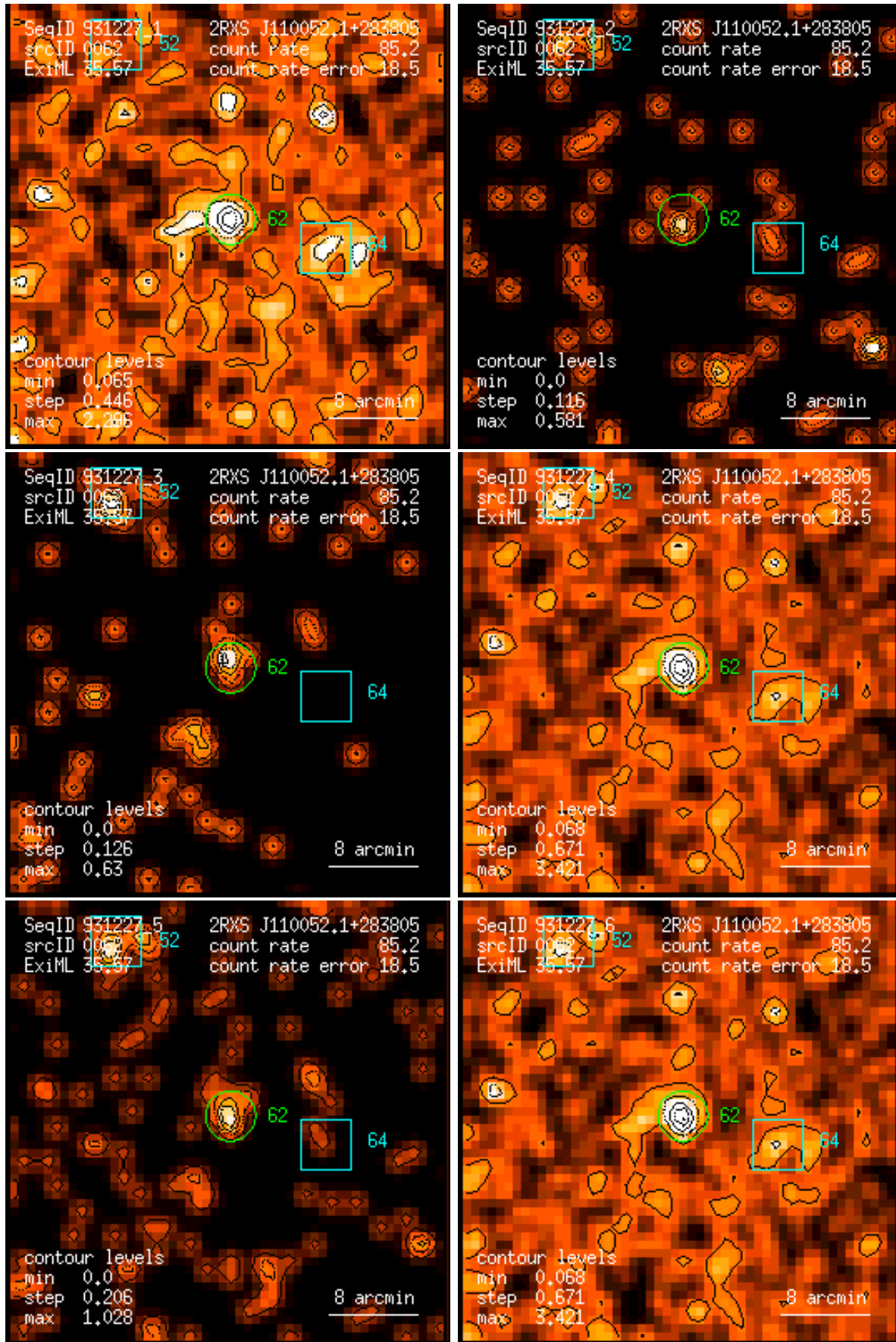
Figure 62: RASS 931227: detection 0062: band rate images, Gaussian filter: (1) PSPC channels 11 – 41, (2) 52 – 90, (3) 91 – 201, (4) 11 – 235, (5) 52 – 201, (6) 11 – 201. Broad band rates in counts/ks. Band rate contour levels in counts/ks/arcmin 2 .
