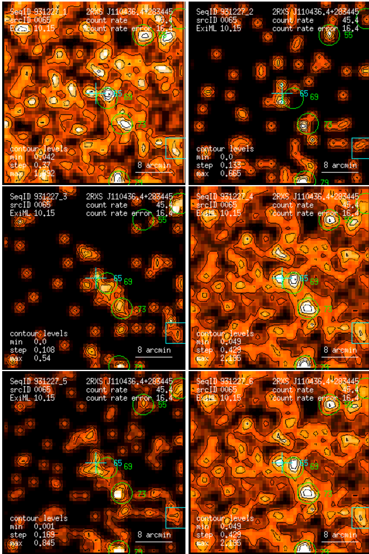
Figure 65: RASS 931227: detection 0065: band rate images, Gaussian filter: (1) PSPC channels 11 – 41, (2) 52 – 90, (3) 91 – 201, (4) 11 – 235, (5) 52 – 201, (6) 11 – 201. Broad band rates in counts/ks. Band rate contour levels in counts/ks/arcmin 2 .
