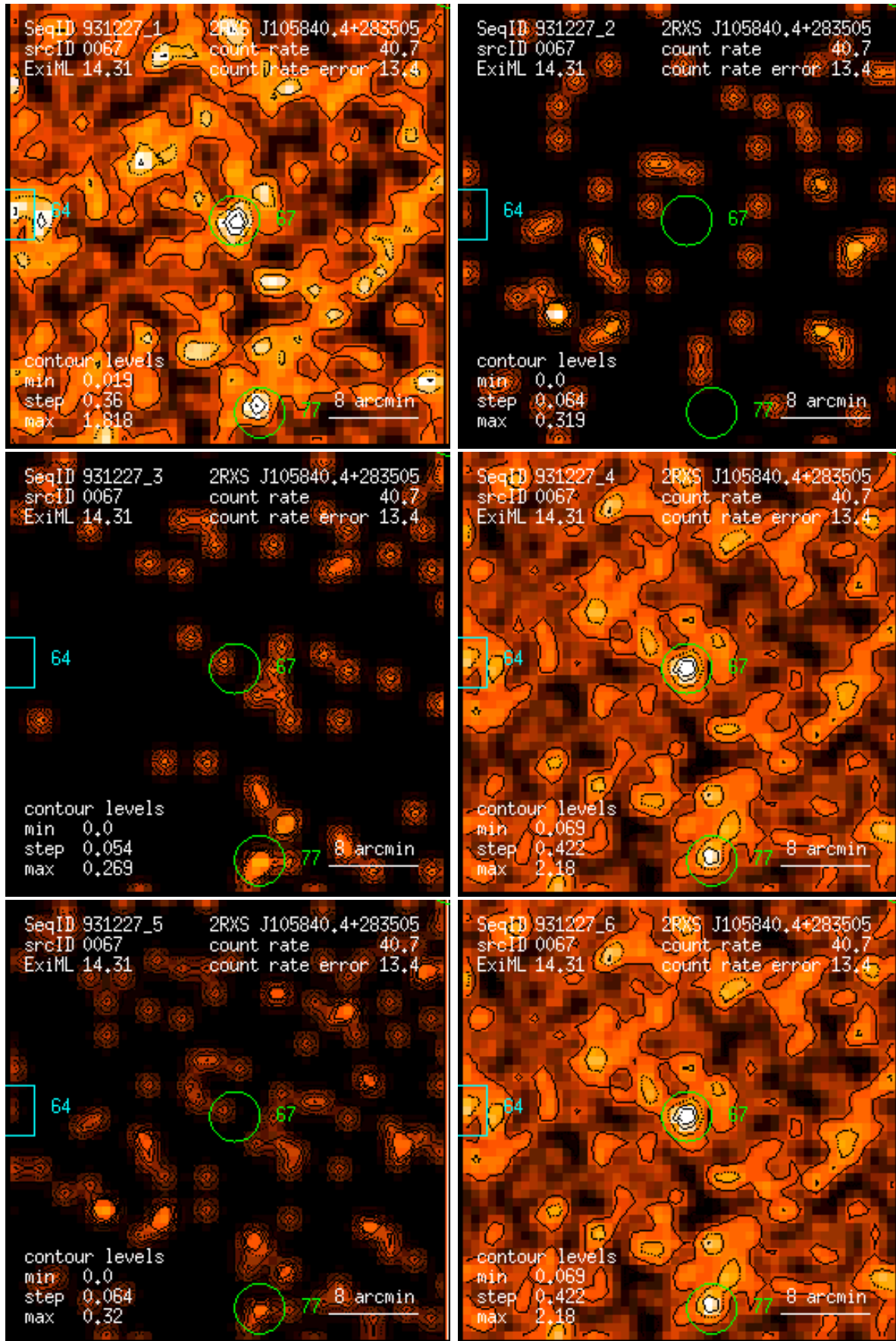
Figure 67: RASS 931227: detection 0067: band rate images, Gaussian filter: (1) PSPC channels 11 – 41, (2) 52 – 90, (3) 91 – 201, (4) 11 – 235, (5) 52 – 201, (6) 11 – 201. Broad band rates in counts/ks. Band rate contour levels in counts/ks/arcmin 2 .
