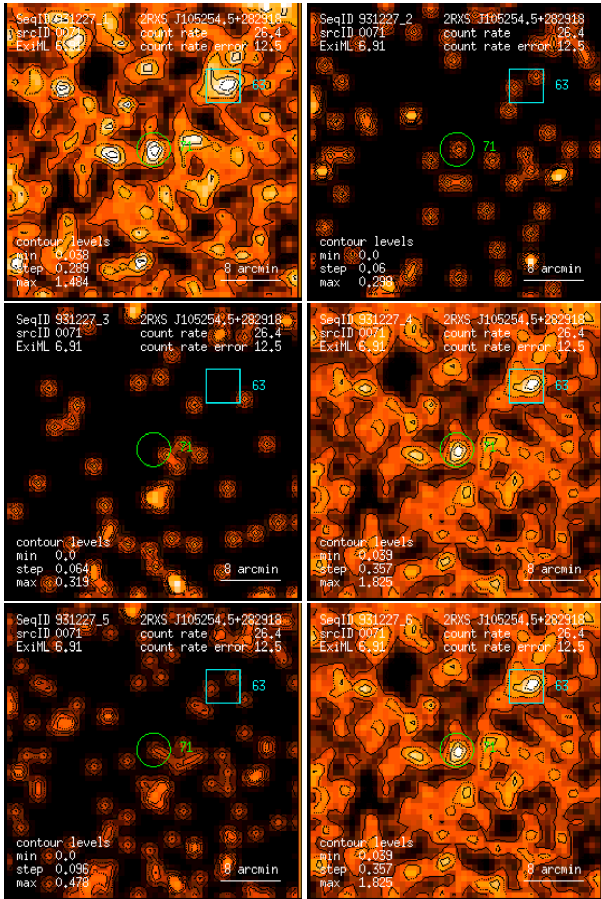
Figure 71: RASS 931227: detection 0071: band rate images, Gaussian filter: (1) PSPC channels 11 – 41, (2) 52 – 90, (3) 91 – 201, (4) 11 – 235, (5) 52 – 201, (6) 11 – 201. Broad band rates in counts/ks. Band rate contour levels in counts/ks/arcmin 2 .
