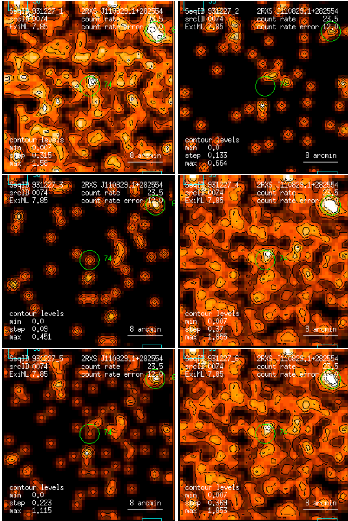
Figure 74: RASS 931227: detection 0074: band rate images, Gaussian filter: (1) PSPC channels 11 – 41, (2) 52 – 90, (3) 91 – 201, (4) 11 – 235, (5) 52 – 201, (6) 11 – 201. Broad band rates in counts/ks. Band rate contour levels in counts/ks/arcmin 2 .
