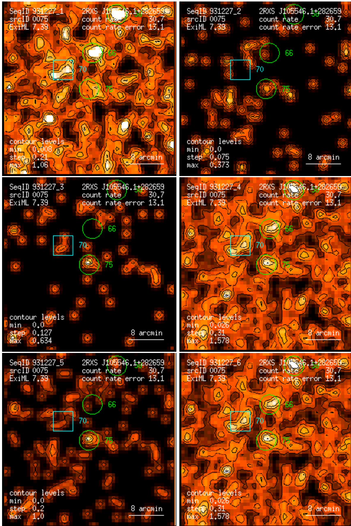
Figure 75: RASS 931227: detection 0075: band rate images, Gaussian filter: (1) PSPC channels 11 – 41, (2) 52 – 90, (3) 91 – 201, (4) 11 – 235, (5) 52 – 201, (6) 11 – 201. Broad band rates in counts/ks. Band rate contour levels in counts/ks/arcmin 2 .
