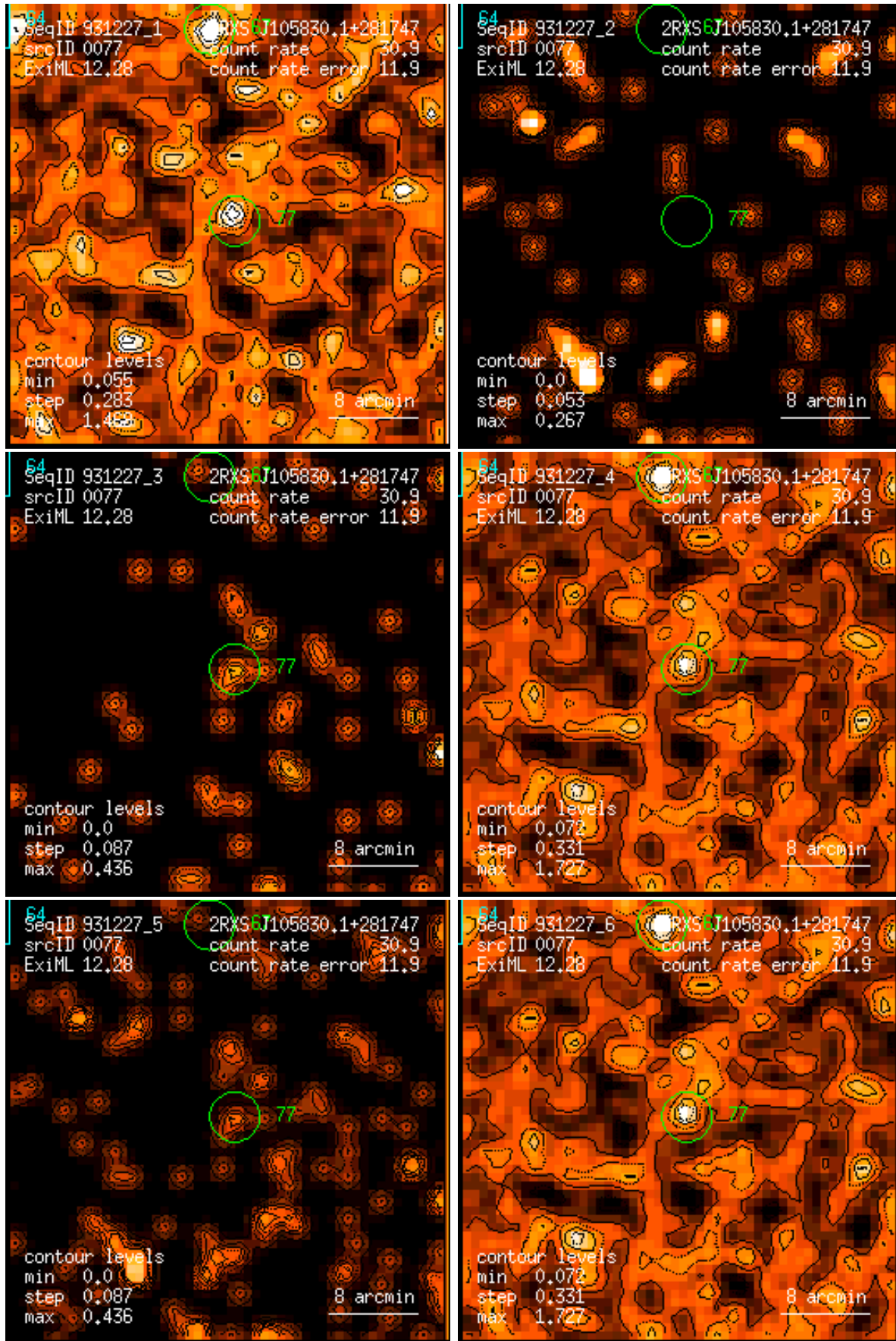
Figure 77: RASS 931227: detection 0077: band rate images, Gaussian filter: (1) PSPC channels 11 – 41, (2) 52 – 90, (3) 91 – 201, (4) 11 – 235, (5) 52 – 201, (6) 11 – 201. Broad band rates in counts/ks. Band rate contour levels in counts/ks/arcmin 2 .
