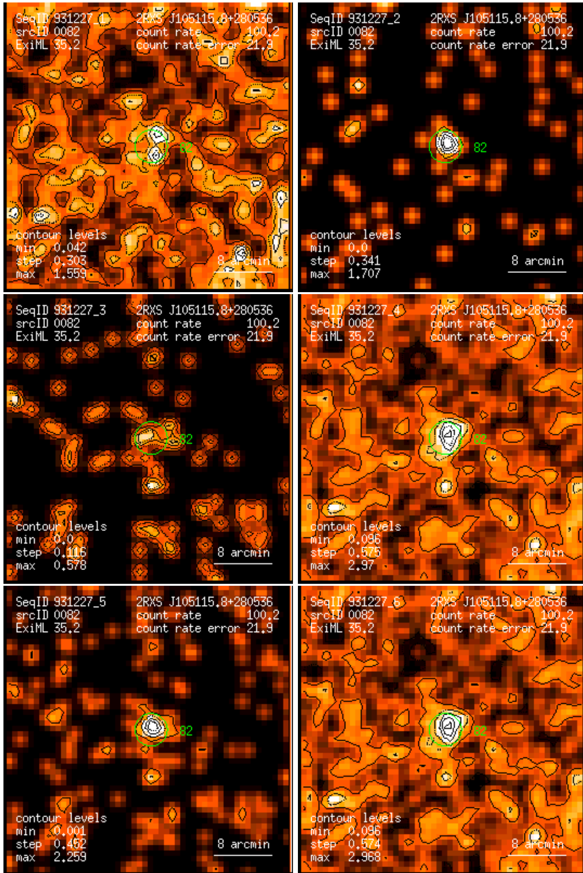
Figure 82: RASS 931227: detection 0082: band rate images, Gaussian filter: (1) PSPC channels 11 – 41, (2) 52 – 90, (3) 91 – 201, (4) 11 – 235, (5) 52 – 201, (6) 11 – 201. Broad band rates in counts/ks. Band rate contour levels in counts/ks/arcmin 2 .
