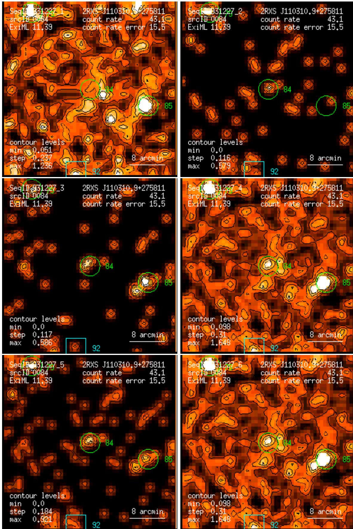
Figure 84: RASS 931227: detection 0084: band rate images, Gaussian filter: (1) PSPC channels 11 – 41, (2) 52 – 90, (3) 91 – 201, (4) 11 – 235, (5) 52 – 201, (6) 11 – 201. Broad band rates in counts/ks. Band rate contour levels in counts/ks/arcmin 2 .
