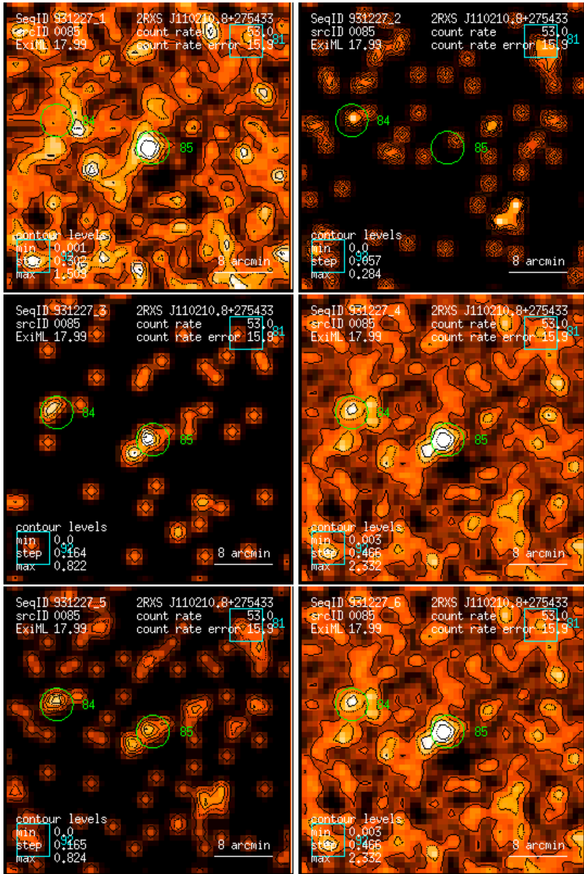
Figure 85: RASS 931227: detection 0085: band rate images, Gaussian filter: (1) PSPC channels 11 – 41, (2) 52 – 90, (3) 91 – 201, (4) 11 – 235, (5) 52 – 201, (6) 11 – 201. Broad band rates in counts/ks. Band rate contour levels in counts/ks/arcmin 2 .
