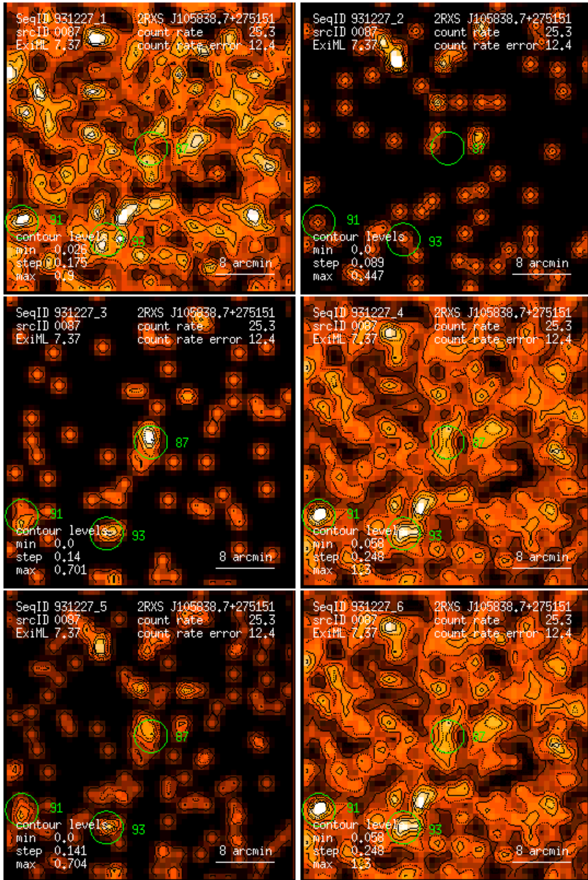
Figure 87: RASS 931227: detection 0087: band rate images, Gaussian filter: (1) PSPC channels 11 – 41, (2) 52 – 90, (3) 91 – 201, (4) 11 – 235, (5) 52 – 201, (6) 11 – 201. Broad band rates in counts/ks. Band rate contour levels in counts/ks/arcmin 2 .
