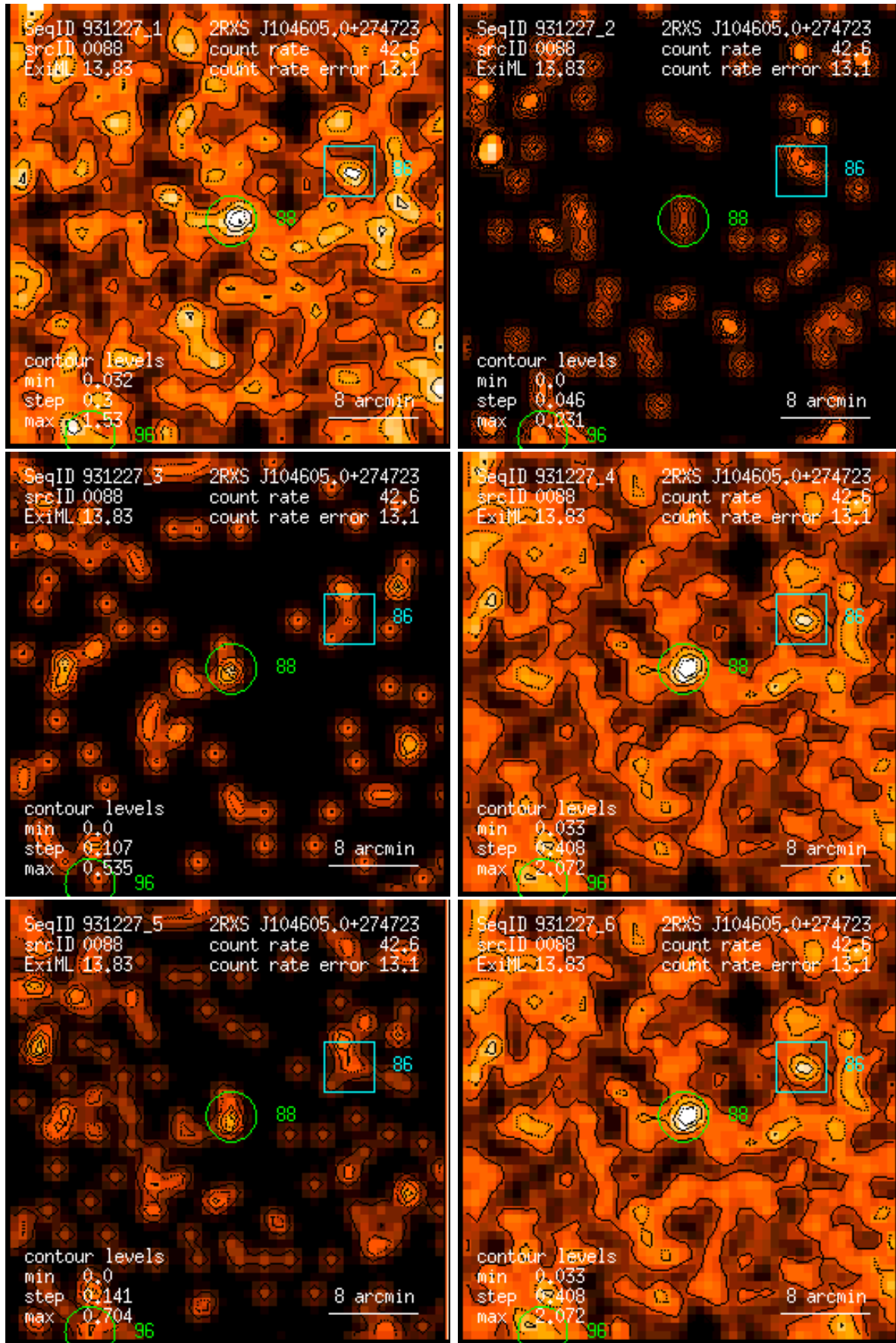
Figure 88: RASS 931227: detection 0088: band rate images, Gaussian filter: (1) PSPC channels 11 – 41, (2) 52 – 90, (3) 91 – 201, (4) 11 – 235, (5) 52 – 201, (6) 11 – 201. Broad band rates in counts/ks. Band rate contour levels in counts/ks/arcmin 2 .
