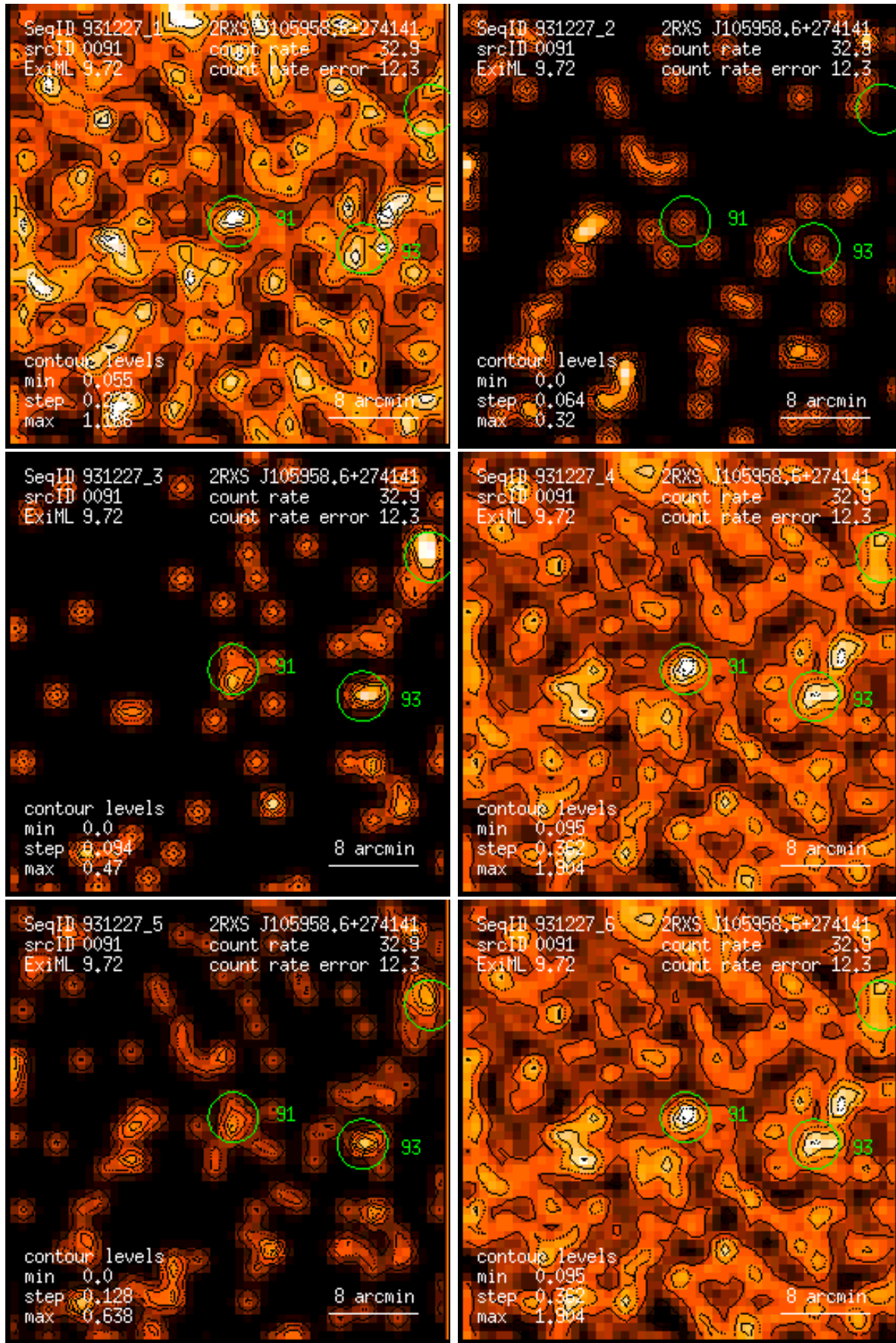
Figure 91: RASS 931227: detection 0091: band rate images, Gaussian filter: (1) PSPC channels 11 – 41, (2) 52 – 90, (3) 91 – 201, (4) 11 – 235, (5) 52 – 201, (6) 11 – 201. Broad band rates in counts/ks. Band rate contour levels in counts/ks/arcmin 2 .
