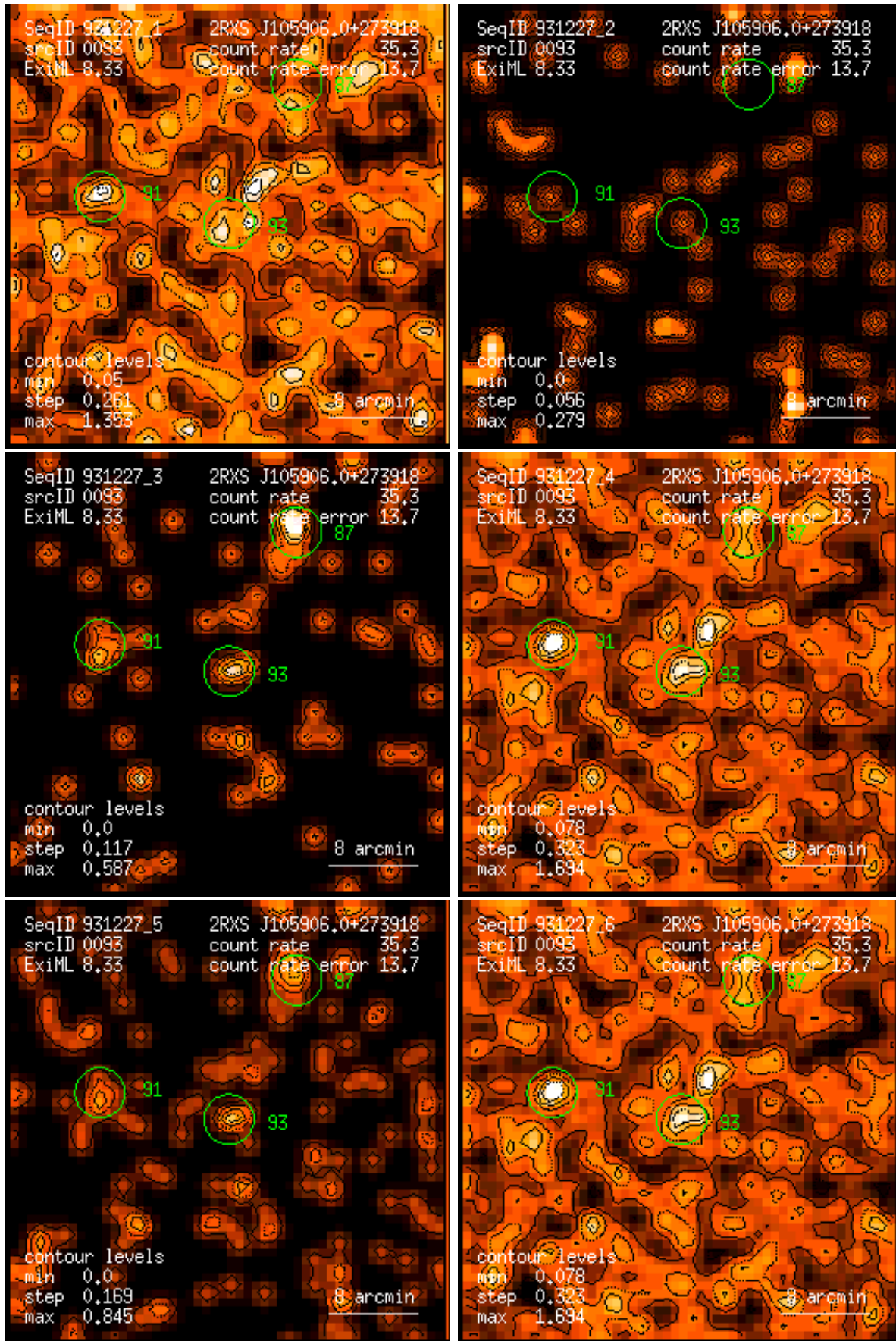
Figure 93: RASS 931227: detection 0093: band rate images, Gaussian filter: (1) PSPC channels 11 – 41, (2) 52 – 90, (3) 91 – 201, (4) 11 – 235, (5) 52 – 201, (6) 11 – 201. Broad band rates in counts/ks. Band rate contour levels in counts/ks/arcmin 2 .
