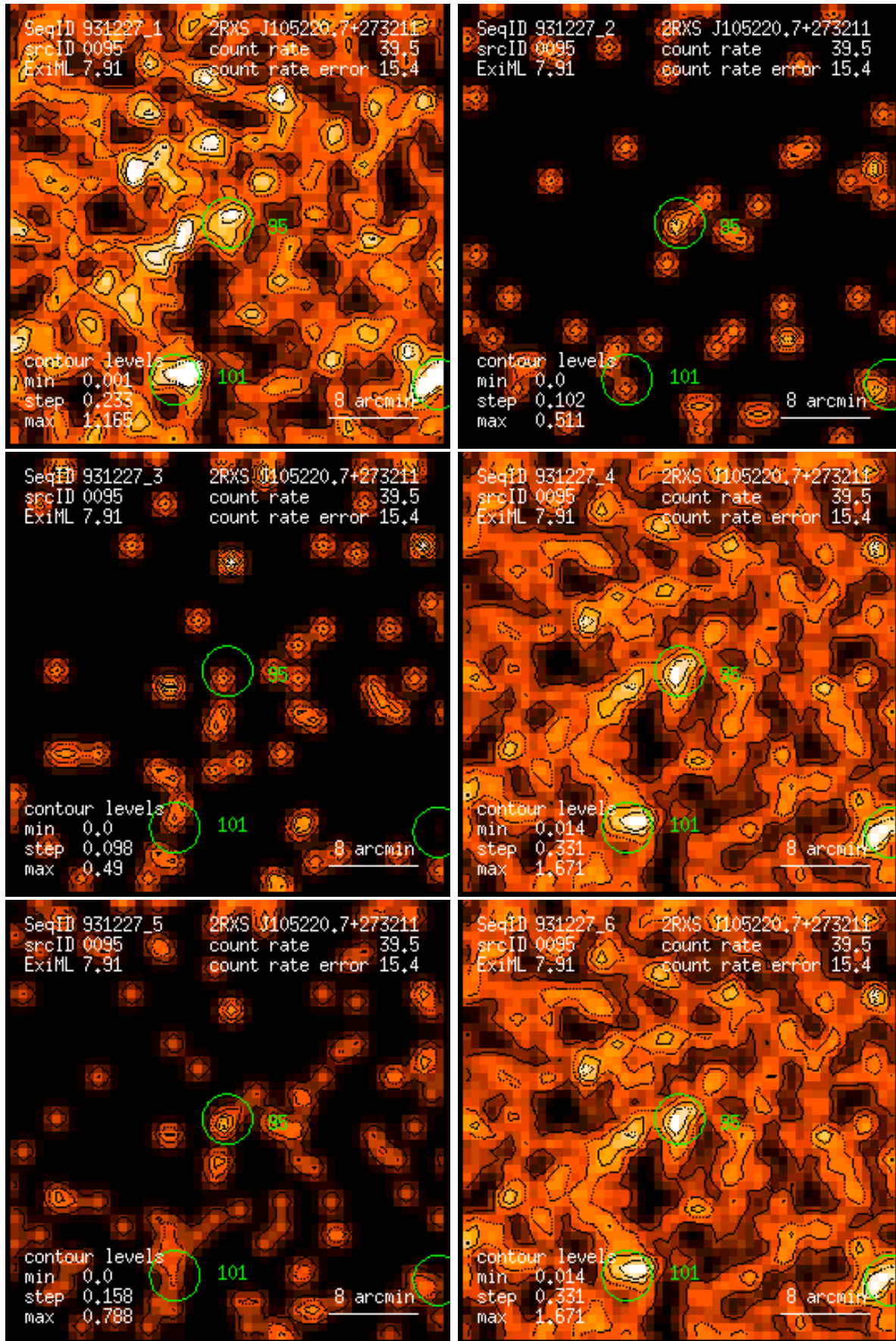
Figure 95: RASS 931227: detection 0095: band rate images, Gaussian filter: (1) PSPC channels 11 – 41, (2) 52 – 90, (3) 91 – 201, (4) 11 – 235, (5) 52 – 201, (6) 11 – 201. Broad band rates in counts/ks. Band rate contour levels in counts/ks/arcmin 2 .
