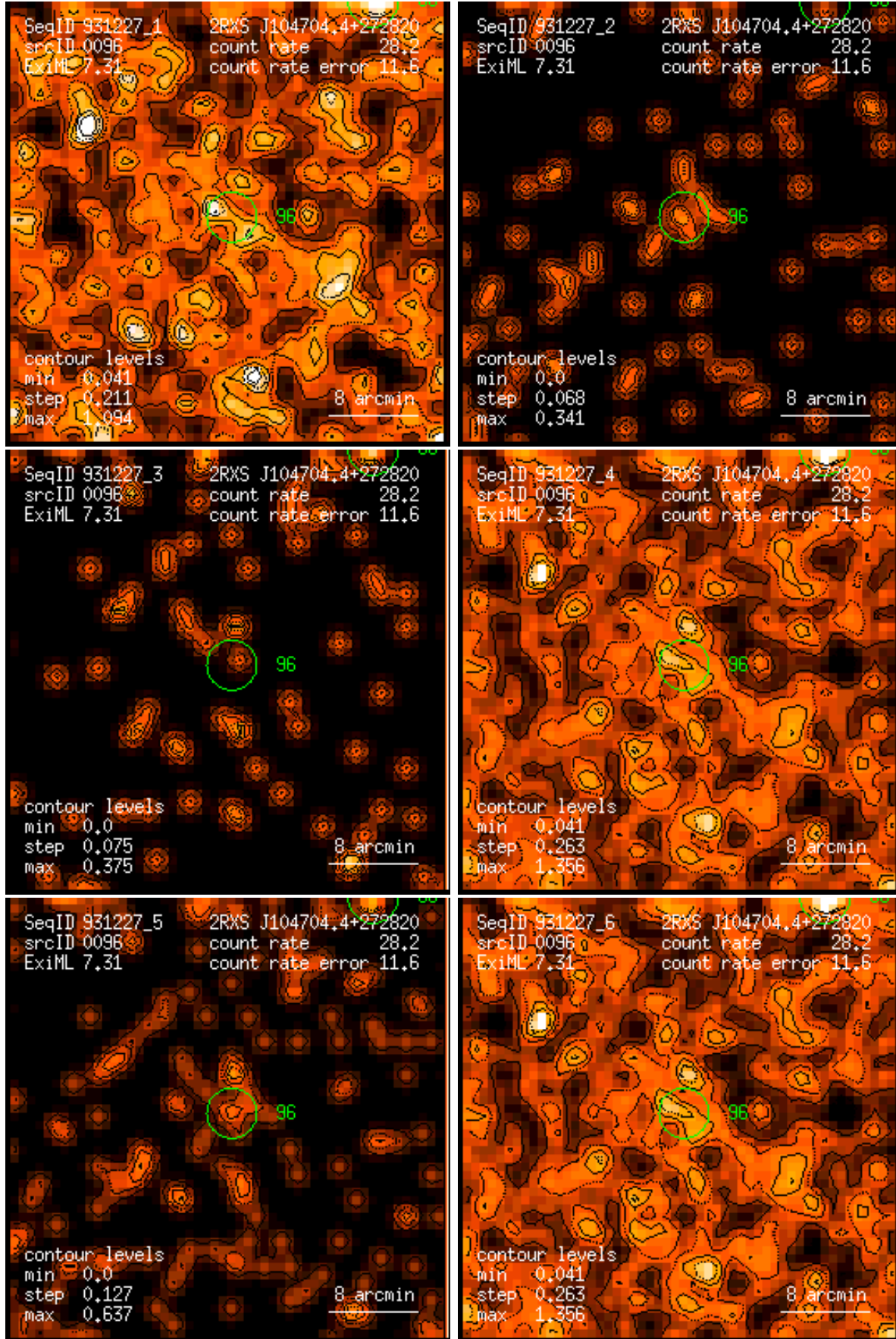
Figure 96: RASS 931227: detection 0096: band rate images, Gaussian filter: (1) PSPC channels 11 – 41, (2) 52 – 90, (3) 91 – 201, (4) 11 – 235, (5) 52 – 201, (6) 11 – 201. Broad band rates in counts/ks. Band rate contour levels in counts/ks/arcmin 2 .
