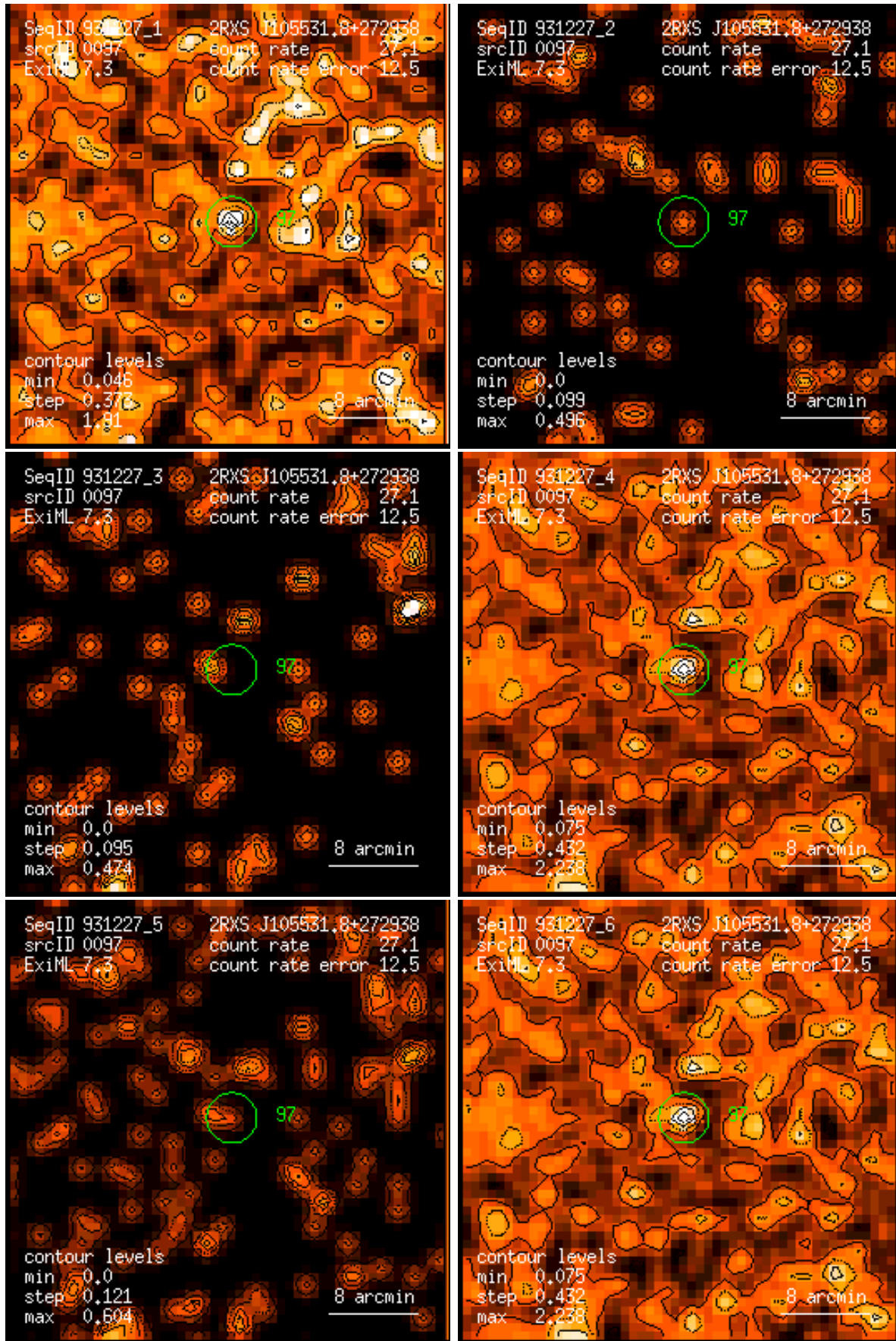
Figure 97: RASS 931227: detection 0097: band rate images, Gaussian filter: (1) PSPC channels 11 – 41, (2) 52 – 90, (3) 91 – 201, (4) 11 – 235, (5) 52 – 201, (6) 11 – 201. Broad band rates in counts/ks. Band rate contour levels in counts/ks/arcmin 2 .
