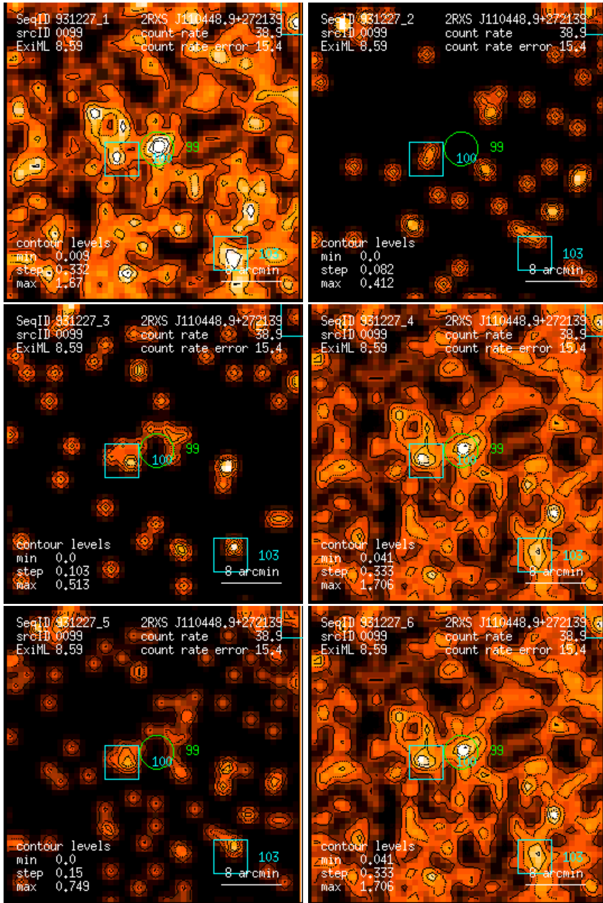
Figure 99: RASS 931227: detection 0099: band rate images, Gaussian filter: (1) PSPC channels 11 – 41, (2) 52 – 90, (3) 91 – 201, (4) 11 – 235, (5) 52 – 201, (6) 11 – 201. Broad band rates in counts/ks. Band rate contour levels in counts/ks/arcmin 2 .
