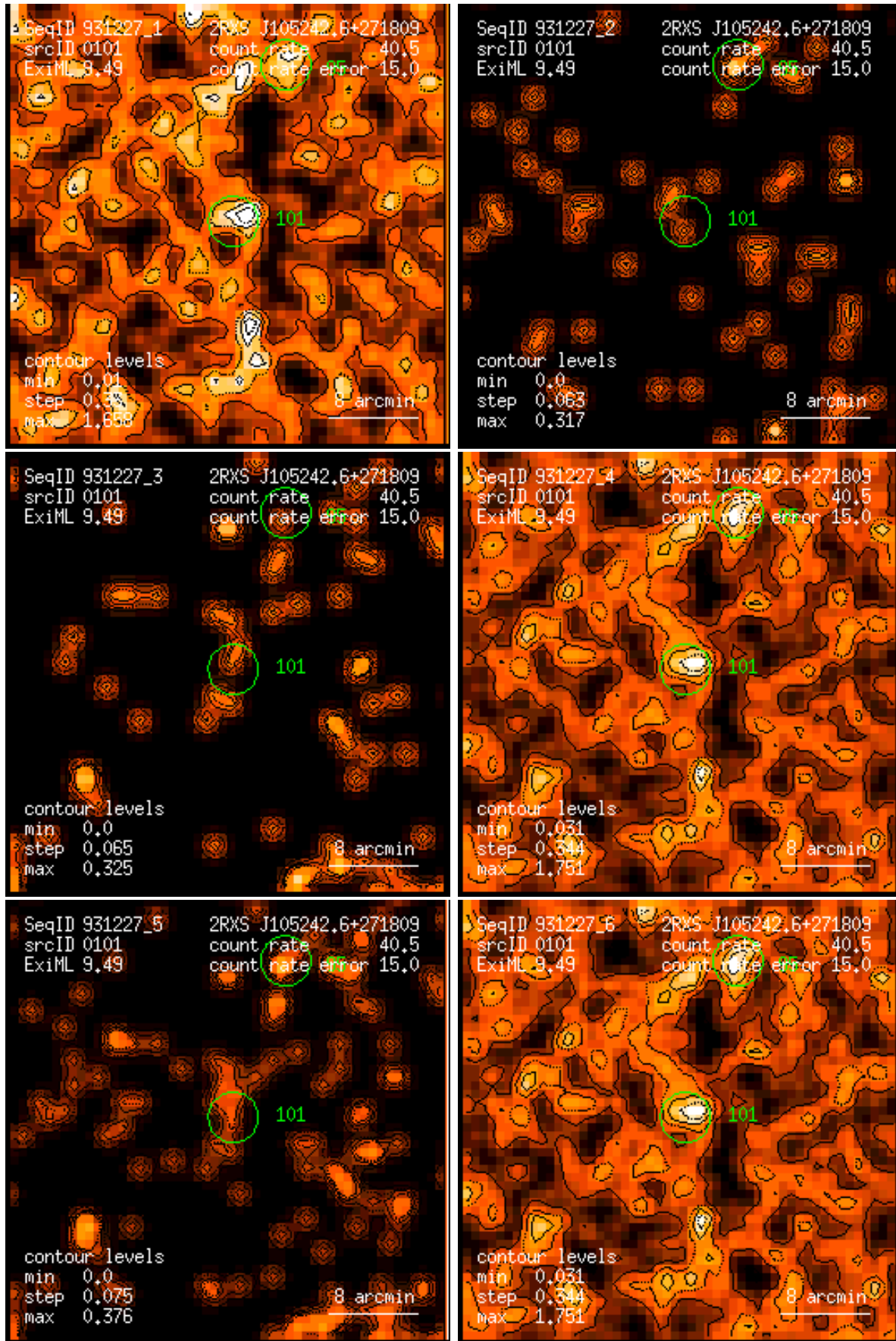
Figure 101: RASS 931227: detection 0101: band rate images, Gaussian filter: (1) PSPPC channels 11 – 41, (2) 52 – 90, (3) 91 – 201, (4) 11 – 235, (5) 52 – 201, (6) 11 – 201. Broad band rates in counts/ks. Band rate contour levels in counts/ks/arcmin 2 .
