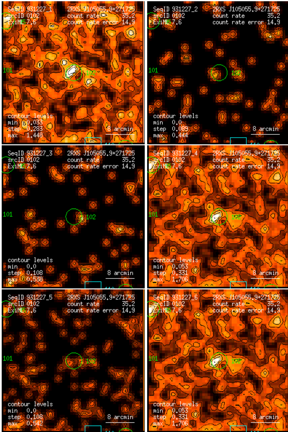
Figure 102: RASS 931227: detection 0102: band rate images, Gaussian filter: (1) PSPC channels 11 – 41, (2) 52 – 90, (3) 91 – 201, (4) 11 – 235, (5) 52 – 201, (6) 11 – 201. Broad band rates in counts/ks. Band rate contour levels in counts/ks/arcmin 2 .
