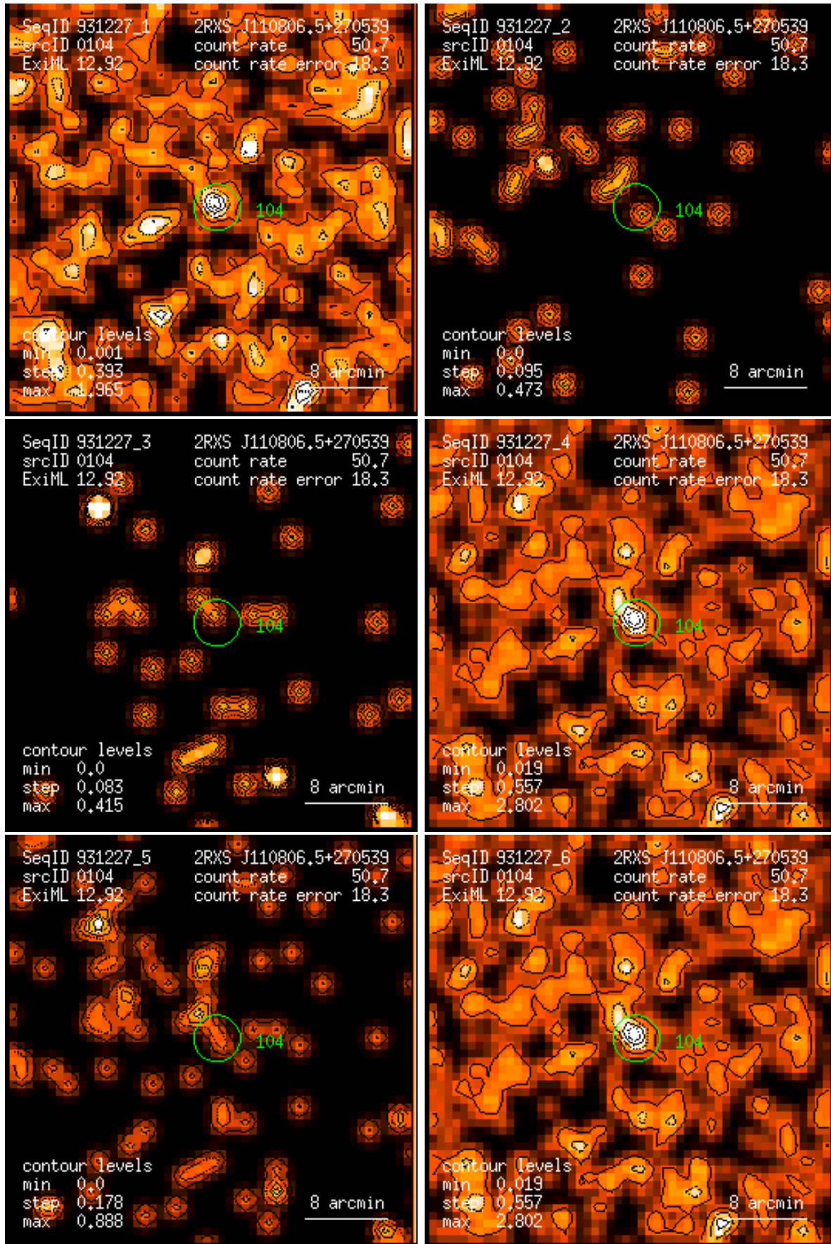
Figure 104: RASS 931227: detection 0104: band rate images, Gaussian filter: (1) PSPC channels 11 – 41, (2) 52 – 90, (3) 91 – 201, (4) 11 – 235, (5) 52 – 201, (6) 11 – 201. Broad band rates in counts/ks. Band rate contour levels in counts/ks/arcmin 2 .
