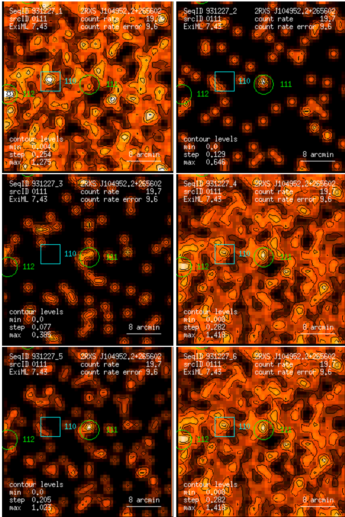
Figure 111: RASS 931227: detection 0111: band rate images, Gaussian filter: (1) PSPC channels 11 – 41, (2) 52 – 90, (3) 91 – 201, (4) 11 – 235, (5) 52 – 201, (6) 11 – 201. Broad band rates in counts/ks. Band rate contour levels in counts/ks/arcmin 2 .
