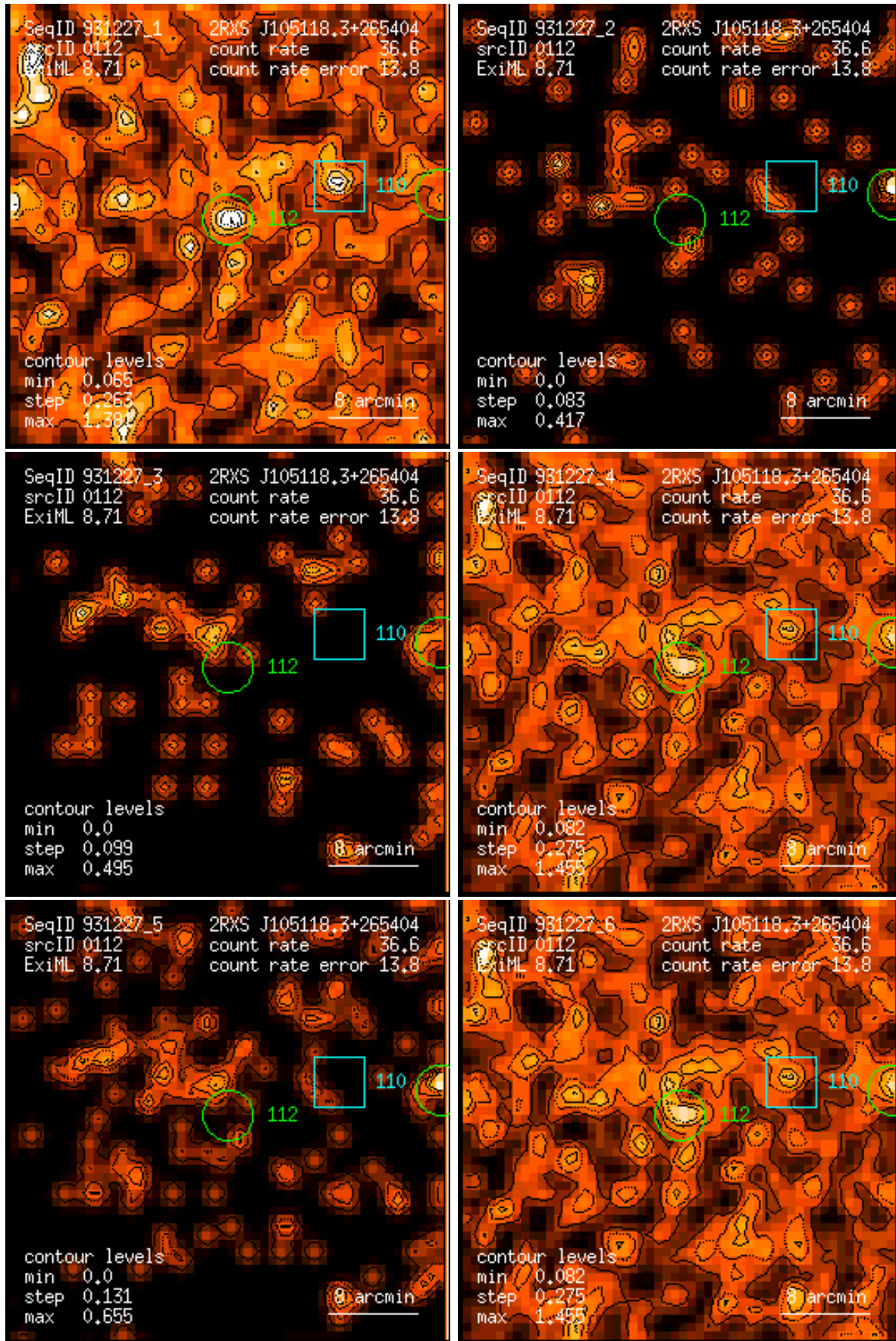
Figure 112: RASS 931227: detection 0112: band rate images, Gaussian filter: (1) PSPC channels 11 – 41, (2) 52 – 90, (3) 91 – 201, (4) 11 – 235, (5) 52 – 201, (6) 11 – 201. Broad band rates in counts/ks. Band rate contour levels in counts/ks/arcmin 2 .
