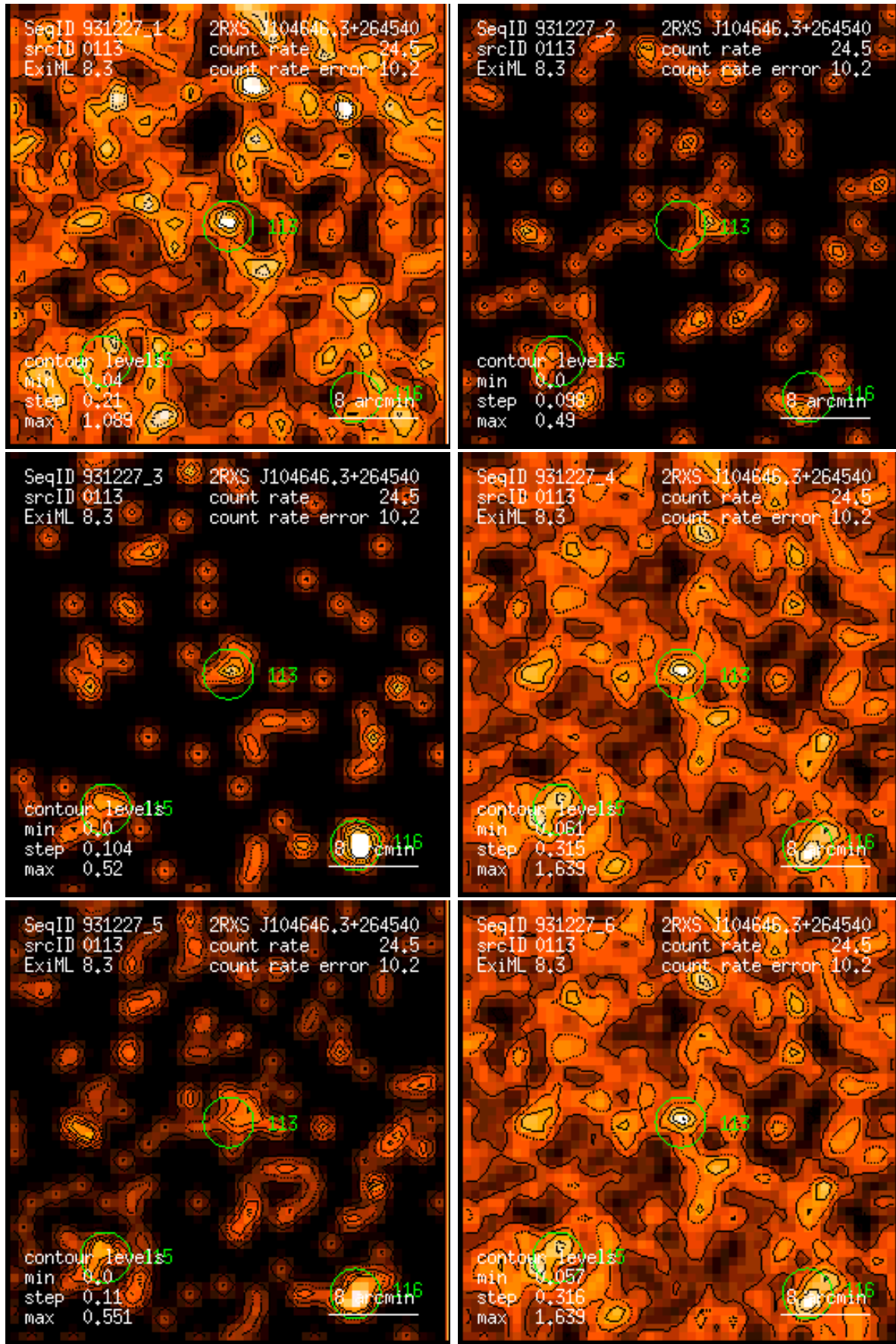
Figure 113: RASS 931227: detection 0113: band rate images, Gaussian filter: (1) PSPC channels 11 – 41, (2) 52 – 90, (3) 91 – 201, (4) 11 – 235, (5) 52 – 201, (6) 11 – 201. Broad band rates in counts/ks. Band rate contour levels in counts/ks/arcmin 2 .
