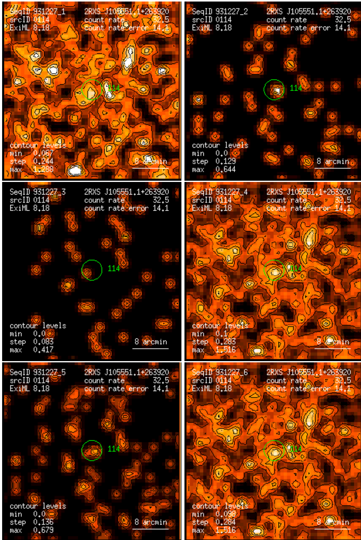
Figure 114: RASS 931227: detection 0114: band rate images, Gaussian filter: (1) PSPC channels 11 – 41, (2) 52 – 90, (3) 91 – 201, (4) 11 – 235, (5) 52 – 201, (6) 11 – 201. Broad band rates in counts/ks. Band rate contour levels in counts/ks/arcmin 2 .
