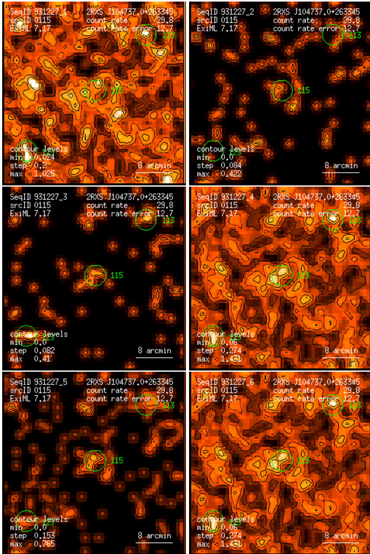
Figure 115: RASS 931227: detection 0115: band rate images, Gaussian filter: (1) PSPC channels 11 – 41, (2) 52 – 90, (3) 91 – 201, (4) 11 – 235, (5) 52 – 201, (6) 11 – 201. Broad band rates in counts/ks. Band rate contour levels in counts/ks/arcmin 2 .
