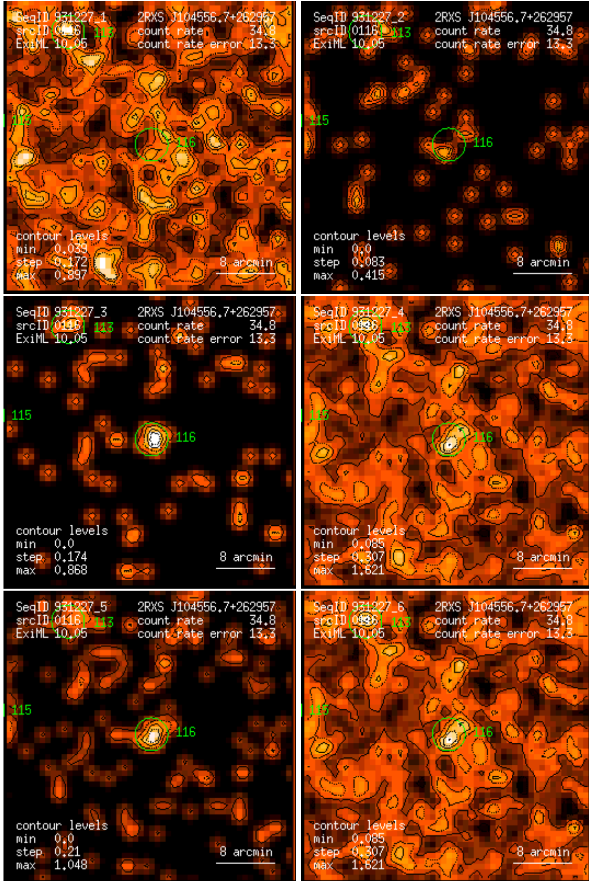
Figure 116: RASS 931227: detection 0116: band rate images, Gaussian filter: (1) PSPC channels 11 – 41, (2) 52 – 90, (3) 91 – 201, (4) 11 – 235, (5) 52 – 201, (6) 11 – 201. Broad band rates in counts/ks. Band rate contour levels in counts/ks/arcmin 2 .
